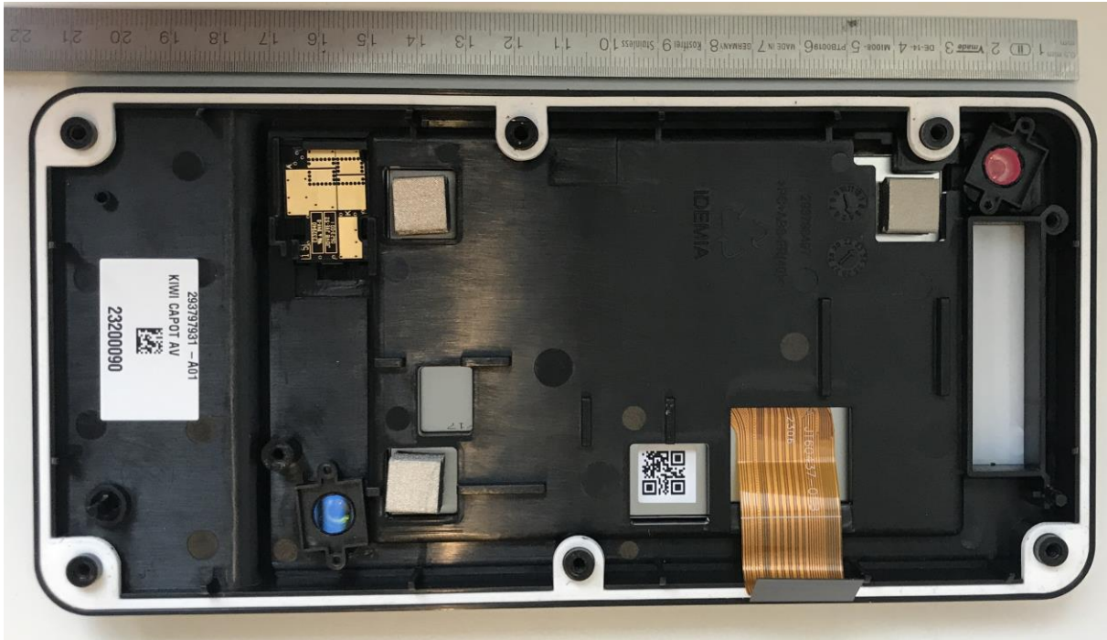
Internal front cover (LCD side):
