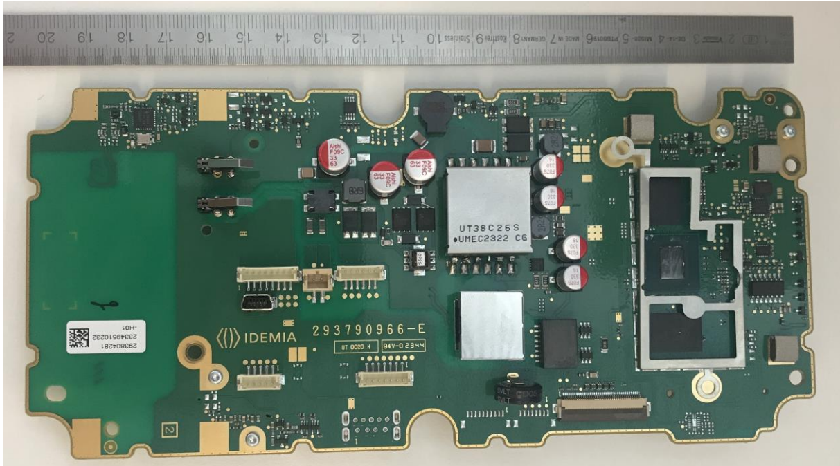
Internal PCB BOARD (from back side)
