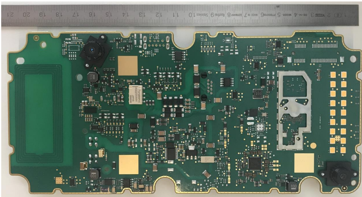
Internal PCB BOARD (from LCD side)
