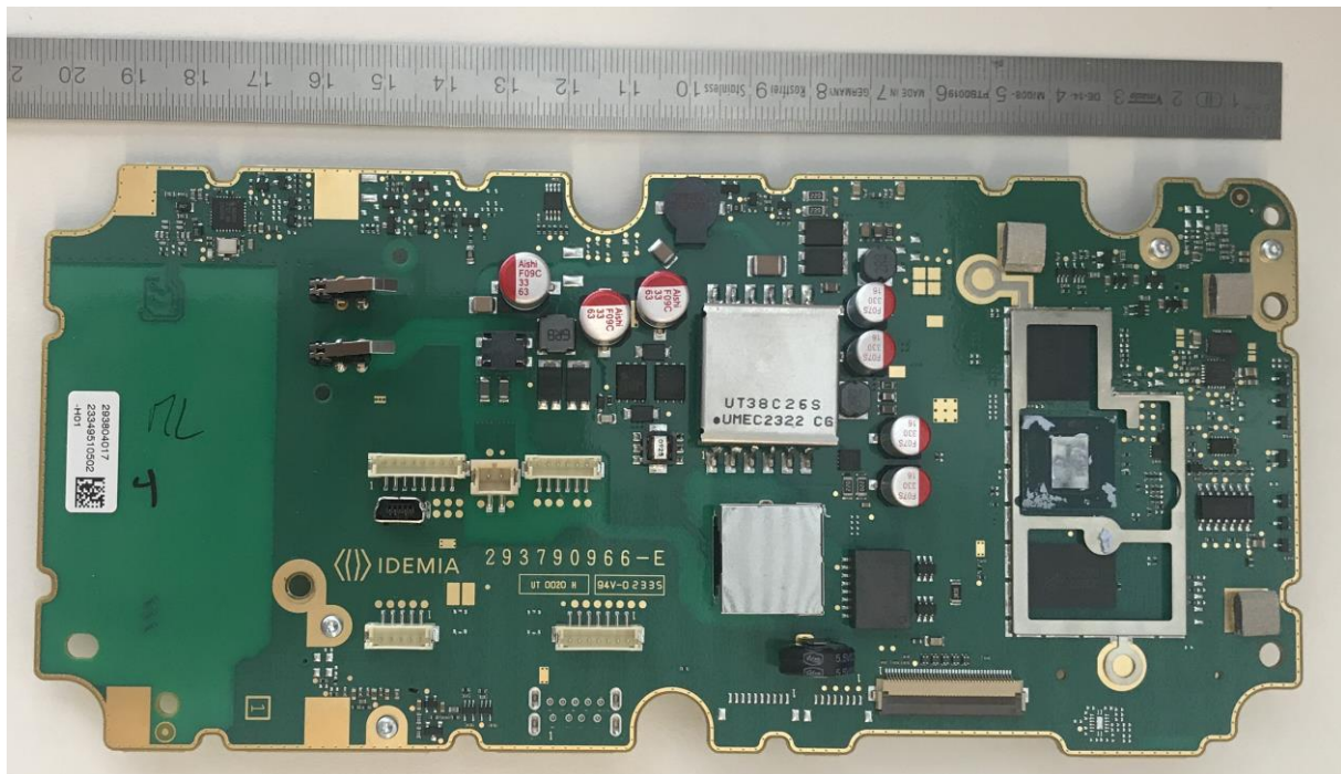
Internal PCB BOARD (from back side)
