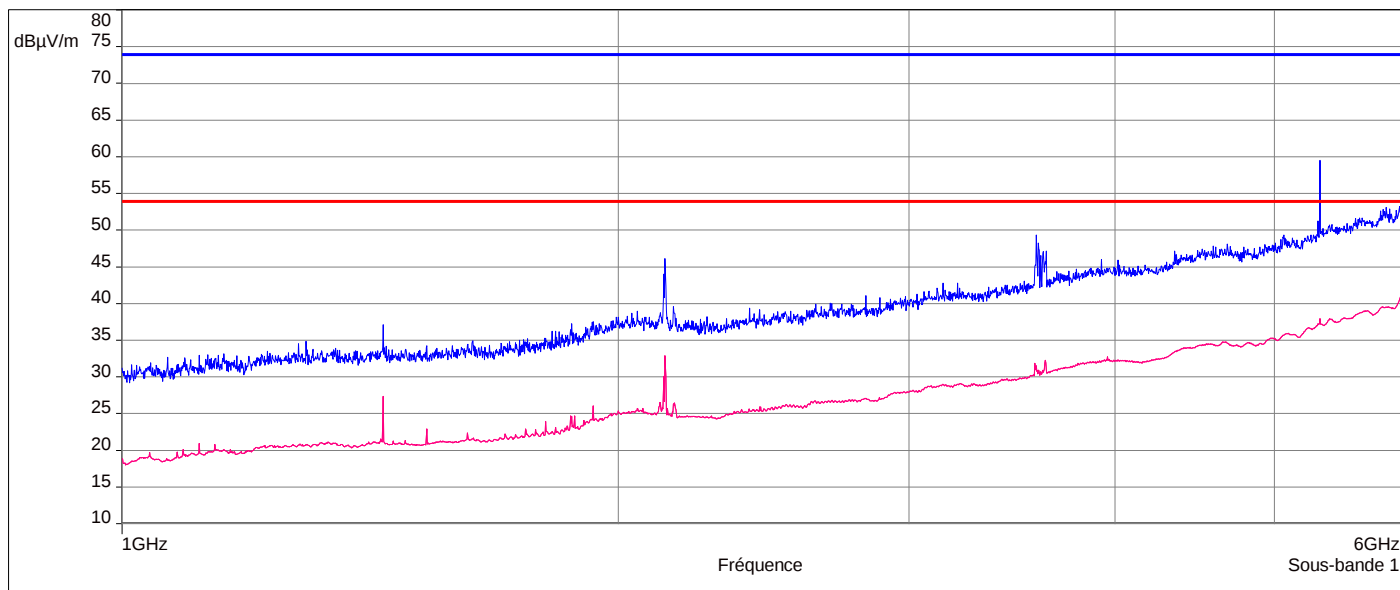
Horizontal Polarization (1-6GHz)
