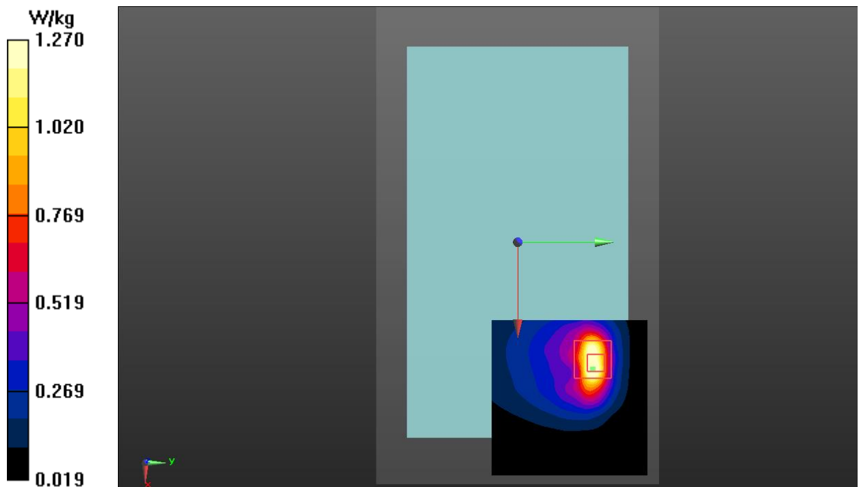
Fig.1 GSM 850 Body
