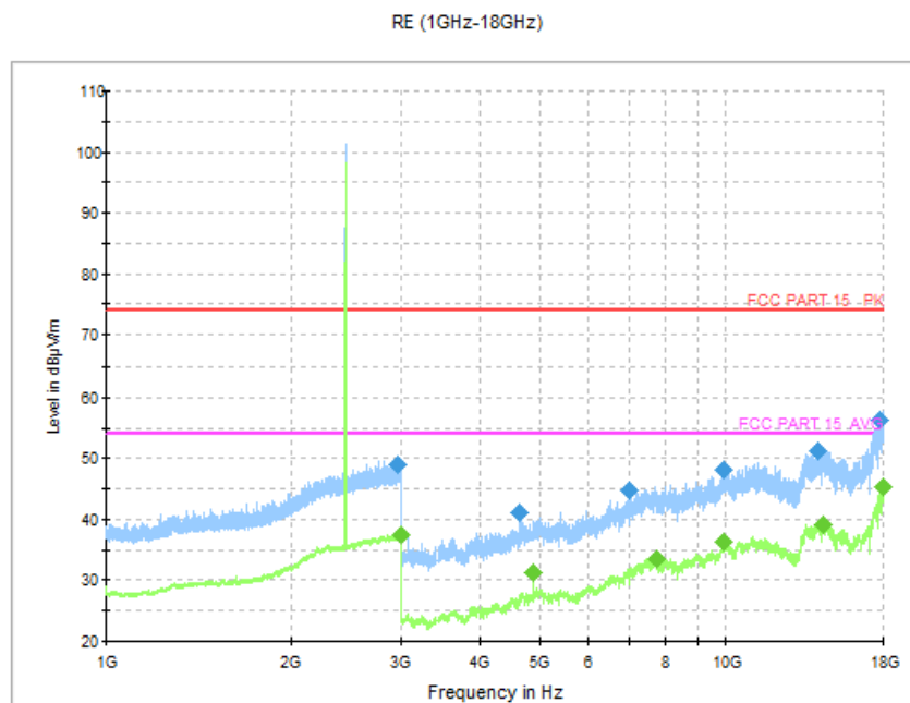
Fig. 53 Radiated Spurious Emission (8DPSK, Ch39, 1 GHz ~18 GHz)
