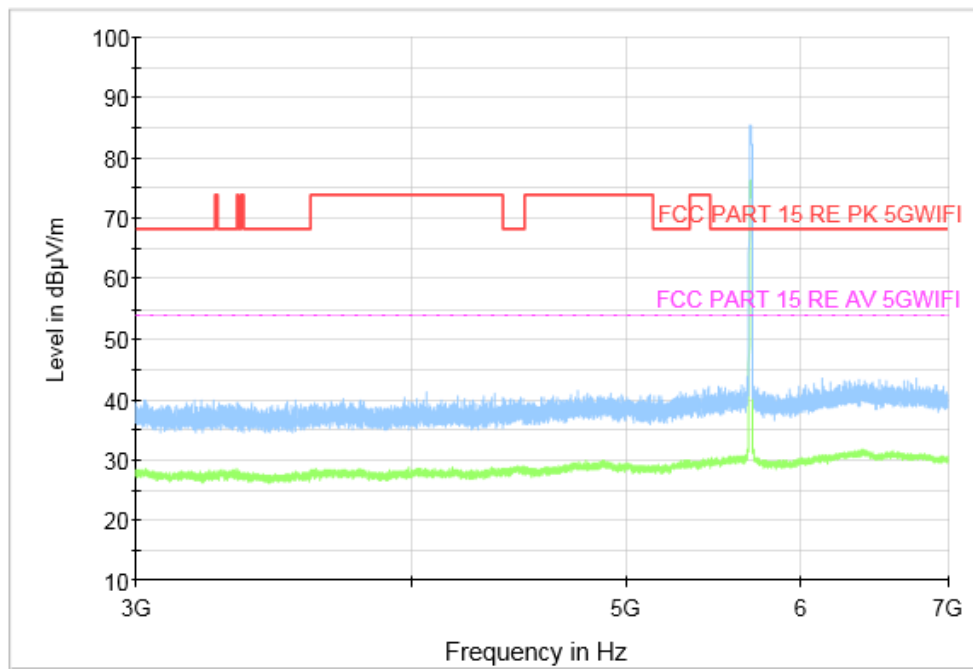
Fig. 79 Transmitter Spurious Emission (802.11a, CH140 5700MHz, 3 GHz-7 GHz)
