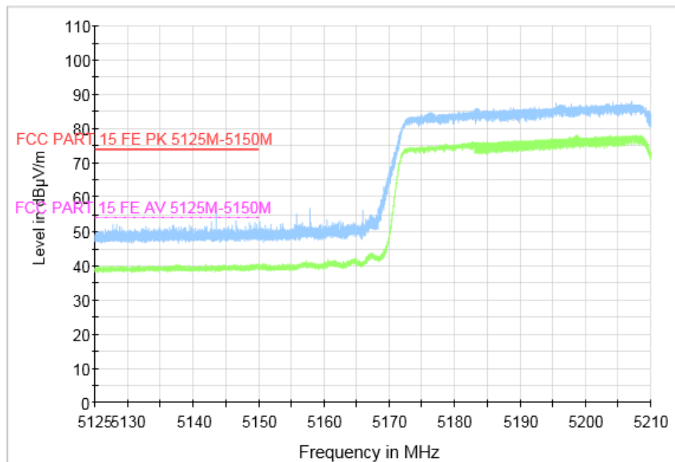
Fig. 59 Band Edges (802.11ac-VHT80, CH42 5210MHz)
