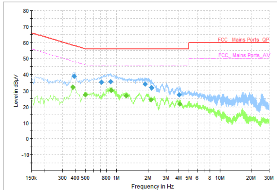
Fig. 121 AC Power line Conducted Emission (Idle, AE1, 120V)
