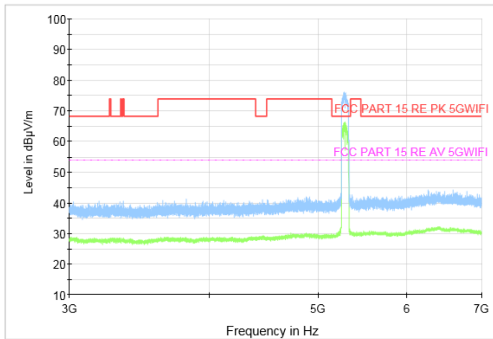
Fig. 107 Transmitter Spurious Emission (802. 11ac-VHT80, CH58 5290MHz, 3 GHz-7 GHz)
