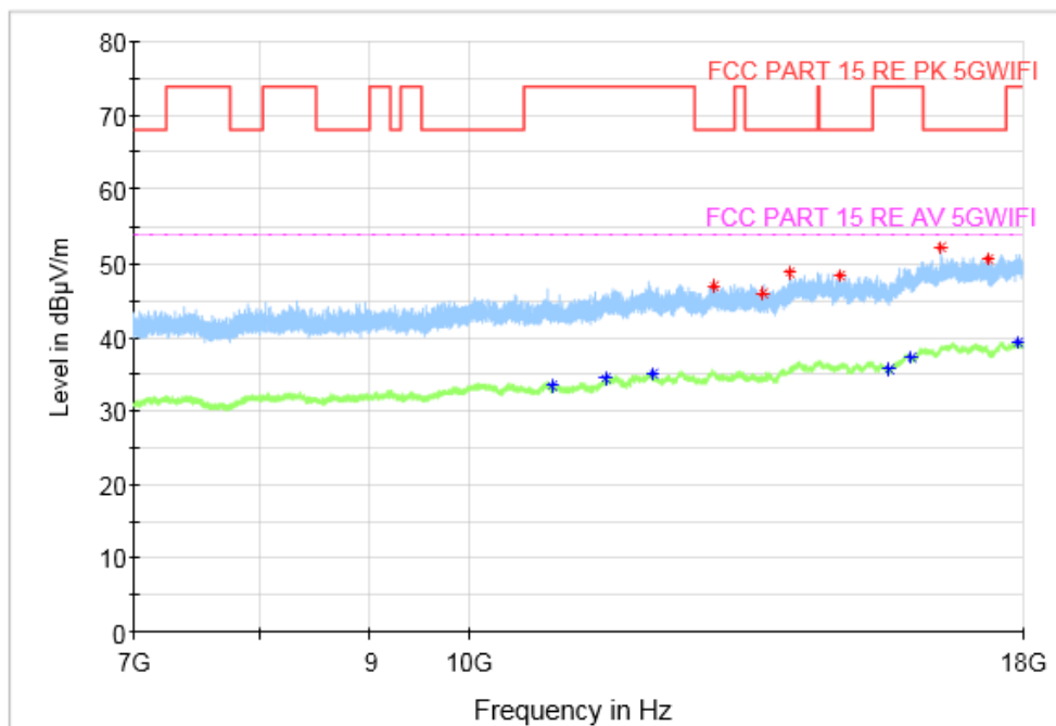
Fig. 110 Transmitter Spurious Emission (802. 11ac-VHT80, CH106 5530MHz, 7 GHz-18 GHz)
