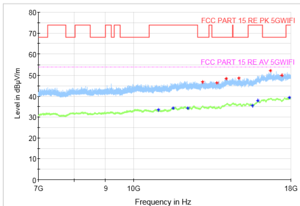
Fig. 112 Transmitter Spurious Emission (802. 11ac-VHT80, CH122 5610MHz, 7 GHz-18 GHz)
