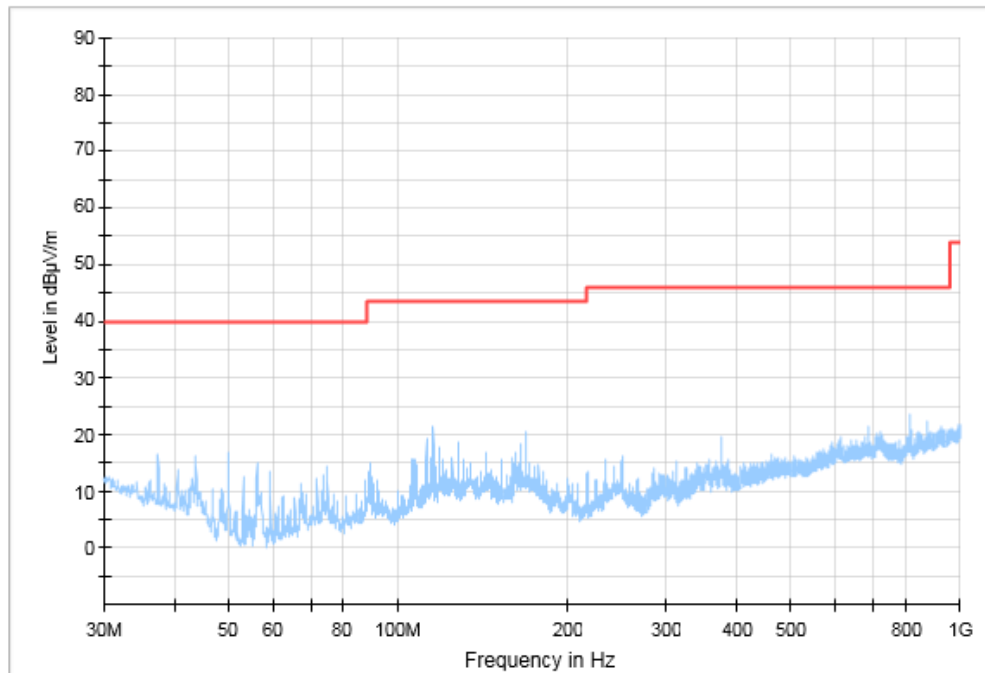
Fig. 115 Transmitter Spurious Emission (All channel, 30MHz~1GHz)
