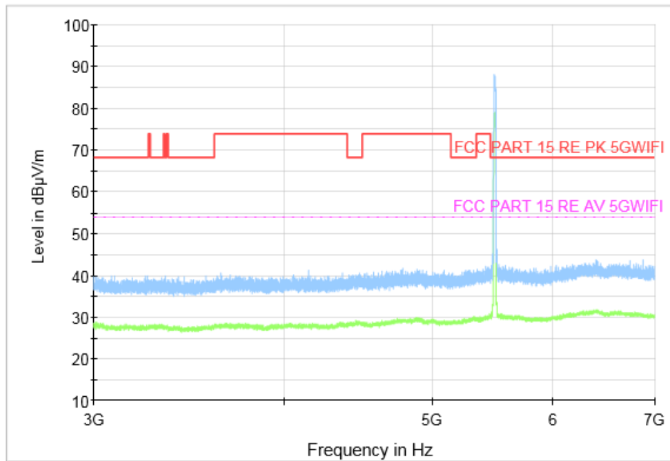
Fig. 75 Transmitter Spurious Emission (802. 11a, CH100 5500MHz, 3 GHz-7 GHz)
