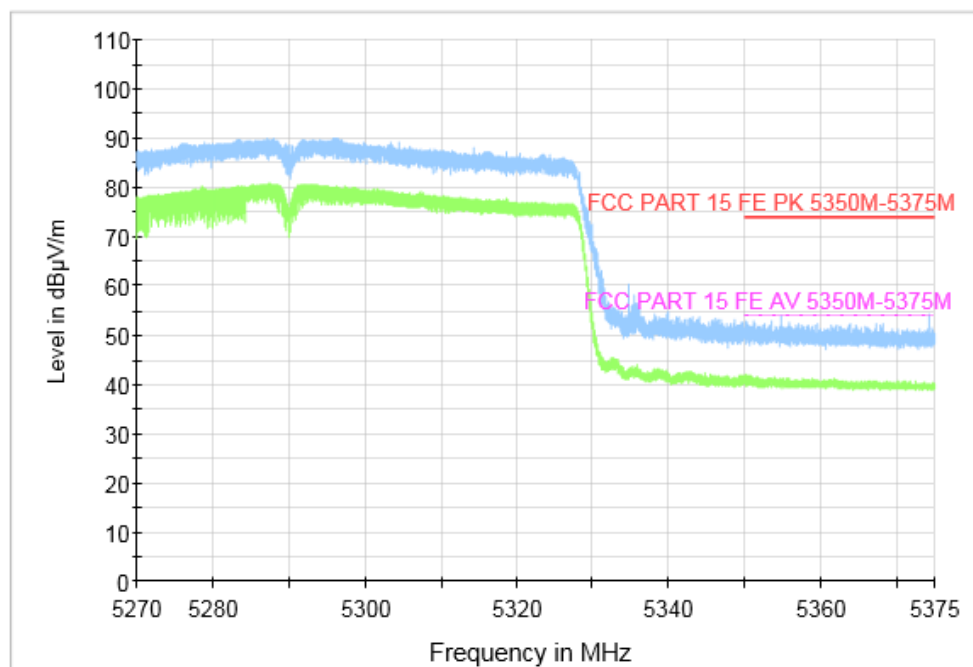
Fig. 60 Band Edges (802.11ac-VHT80, CH58 5290MHz)
