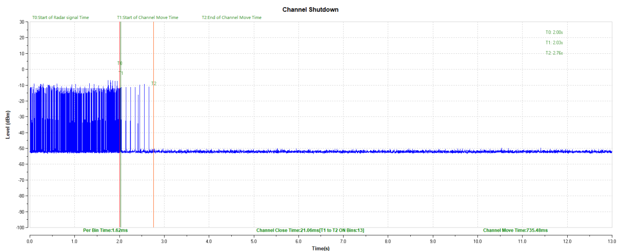
Fig.2 Channel Move Time & Channel Closing Transmission Time (HT80 Frequency Band: 5470MHz~5725MHz)
