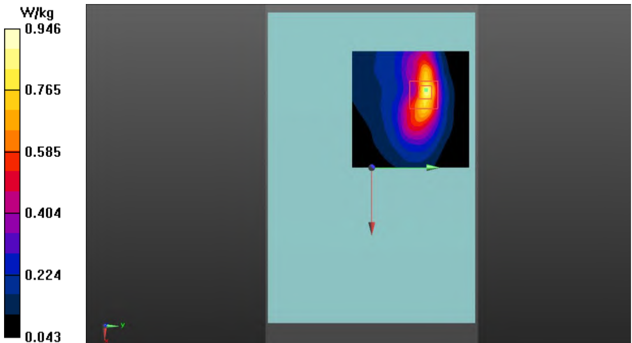
Fig.1 GSM 850 Body
