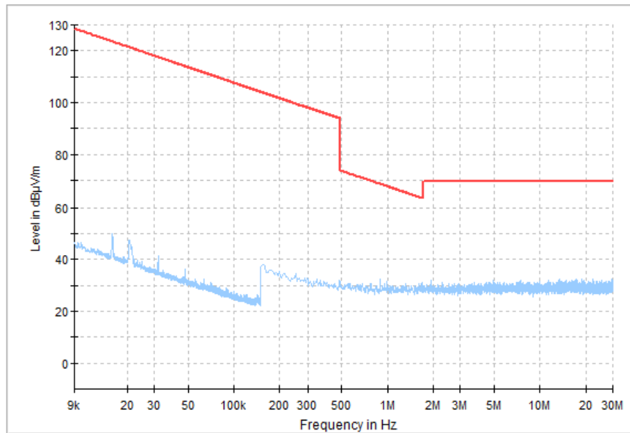
Fig.17 Radiated Spurious Emission (All Channels, 9 kHz-30 MHz), LE
