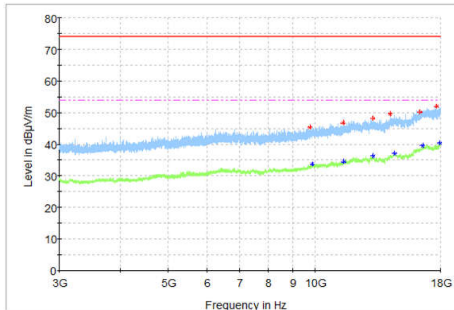
Fig.12 Radiated Spurious Emission (Ch0, 3 GHz ~18 GHz), LE 1M
