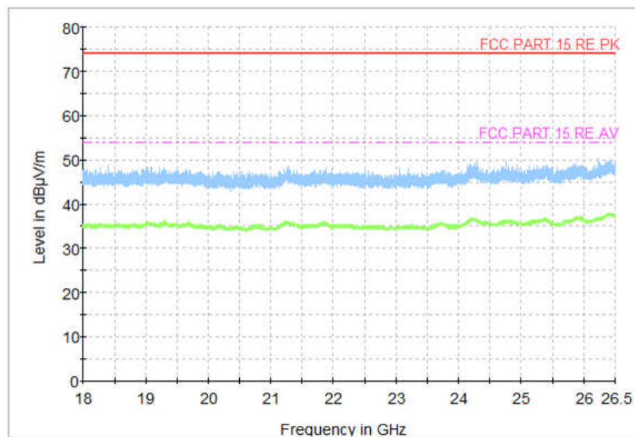
Fig.20 Radiated Spurious Emission (All Channels, 18 GHz-26.5 GHz), LE
