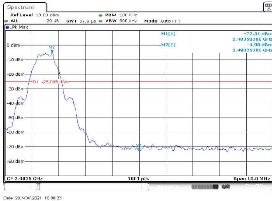
Fig.8 Band Edges (Ch 39), LE 1M
