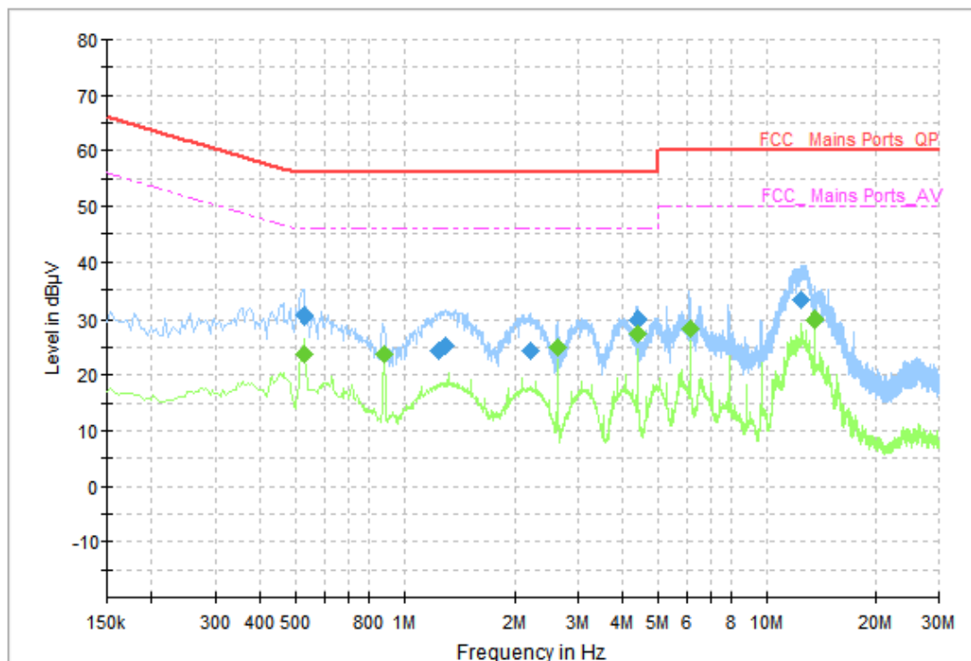
Fig.22 AC Power line Conducted Emission (Idle), LE
