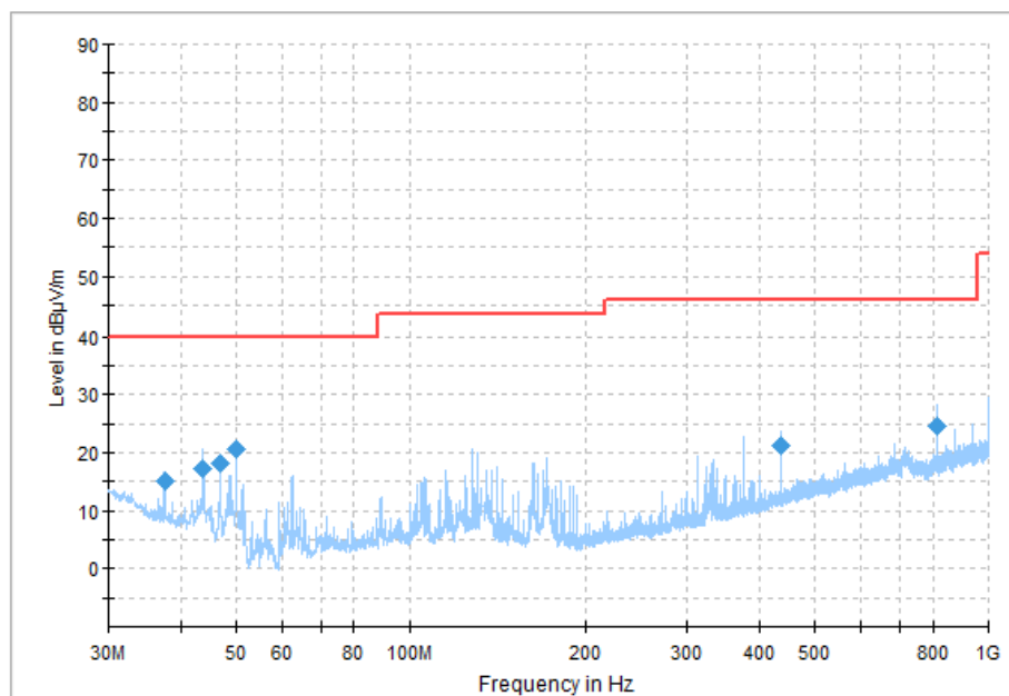
Fig.18 Radiated Spurious Emission (All Channels, 30 MHz-1 GHz), LE
