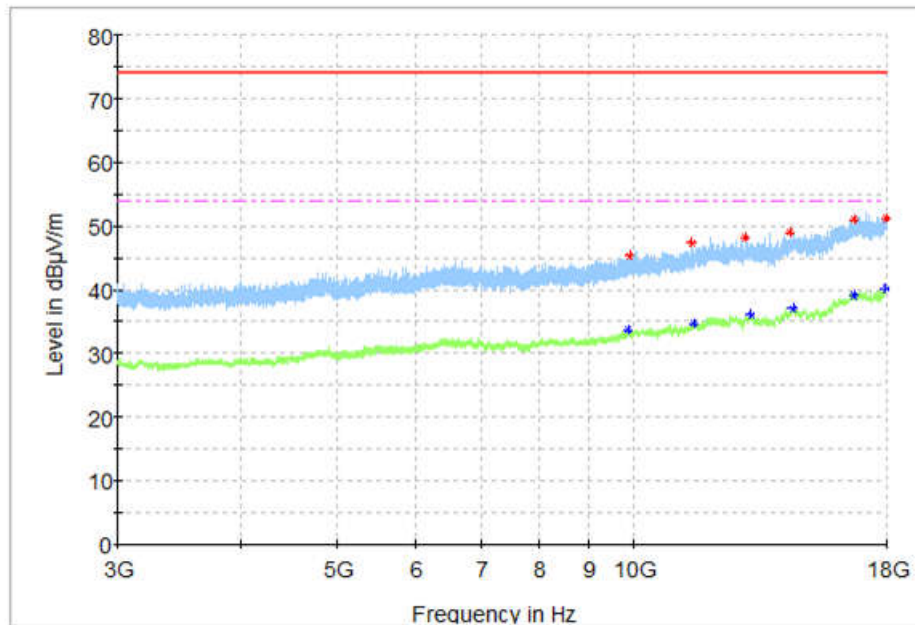
Fig.13 Radiated Spurious Emission (Ch19, 3 GHz ~18 GHz), LE 1M
