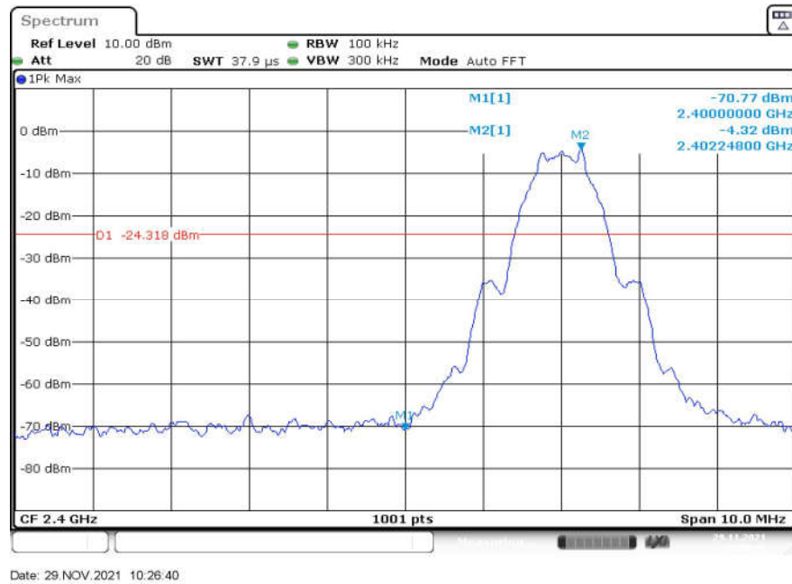
Fig.7 Band Edges (Ch 0), LE 1M
