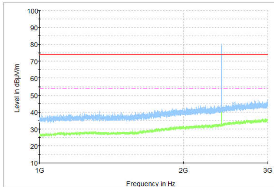
Fig.19 Radiated Spurious Emission (All Channels, 1 GHz-3 GHz), LE
