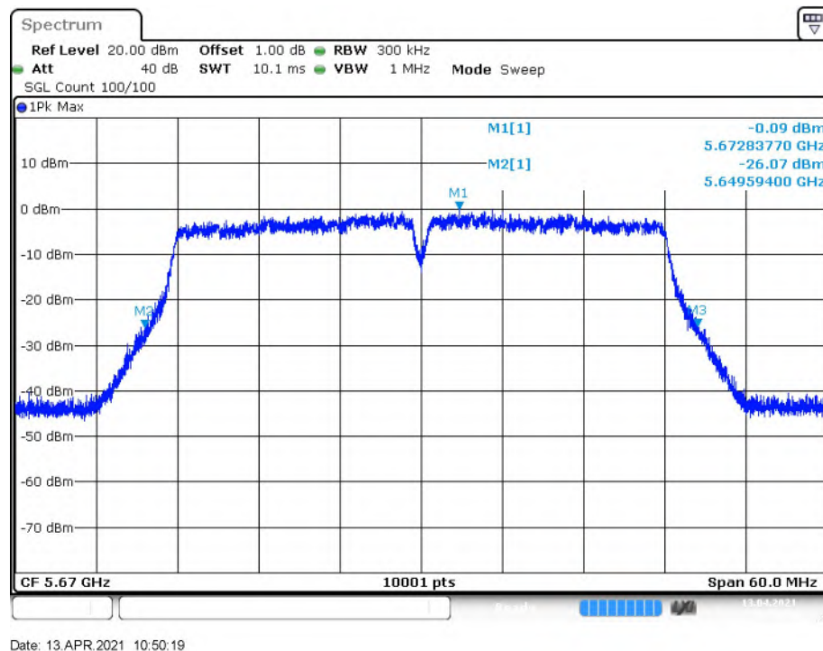
Fig. 16 Occupied 26dB Bandwidth (802.11n-HT40, 5670MHz)
