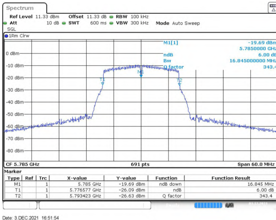
Fig. 22 Occupied 6dB Bandwidth (802.11a, 5785MHz)
