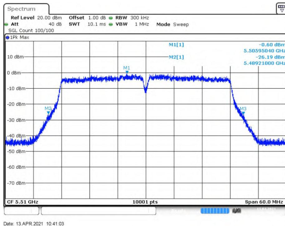
Fig. 14 Occupied 26dB Bandwidth (802.11n-HT40, 5510MHz)
