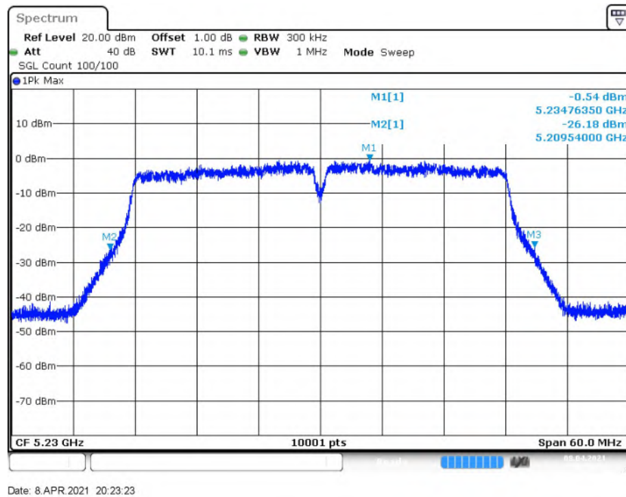
Fig. 11 Occupied 26dB Bandwidth (802.11n-HT40, 5230MHz)
