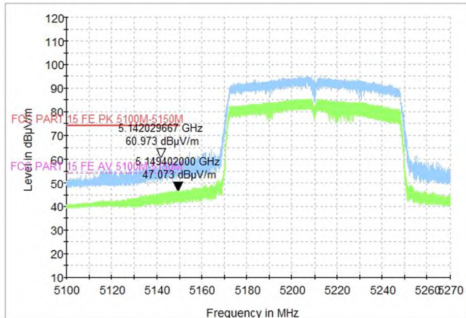
Fig. 63 Band Edges (802.11ac-VHT80, CH42 5210MHz)
