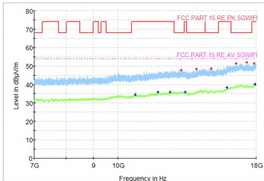
Fig. 72 Transmitter Spurious Emission (802.11a, CH64 5320MHz, 7 GHz-18 GHz)
