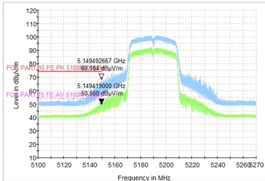
Fig. 57 Band Edges (802.11n-HT40, CH38 5190MHz)
