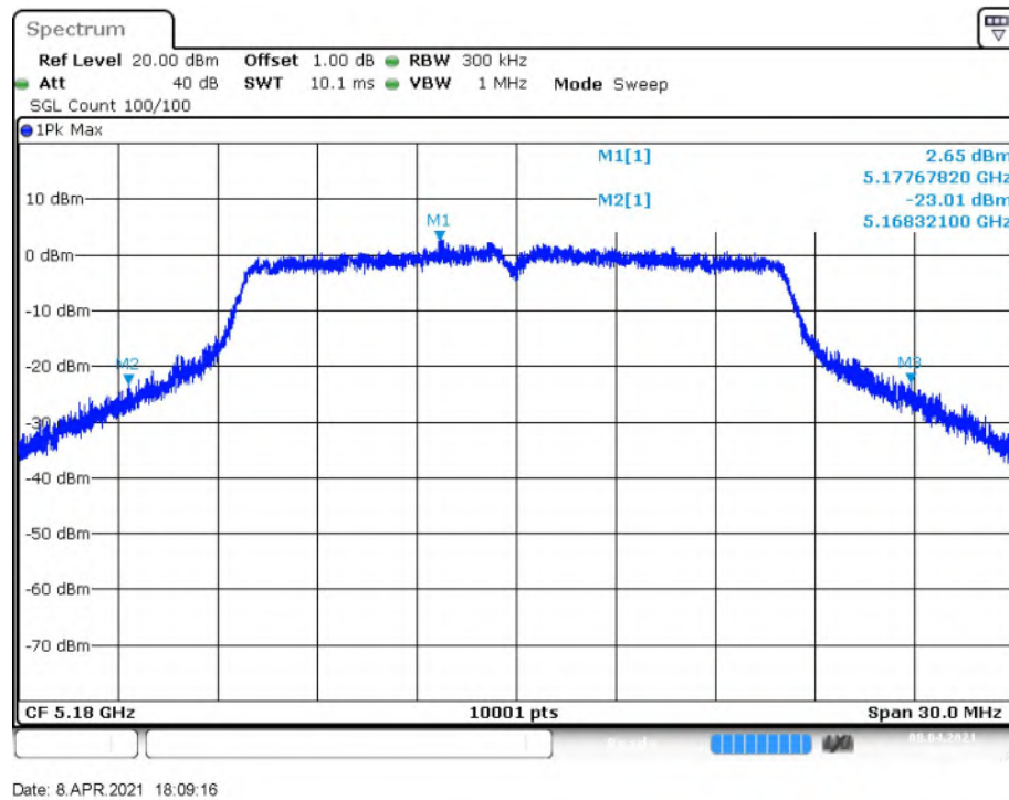
Fig. 1 Occupied 26dB Bandwidth (802.11a, 5180MHz)
