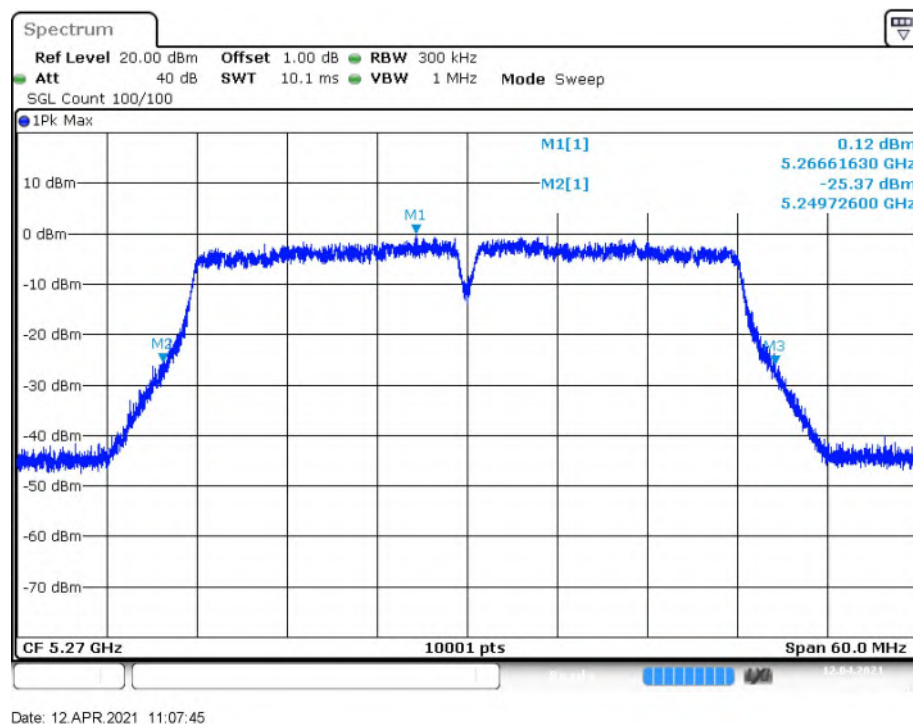
Fig. 12 Occupied 26dB Bandwidth (802.11n-HT40, 5270MHz)
