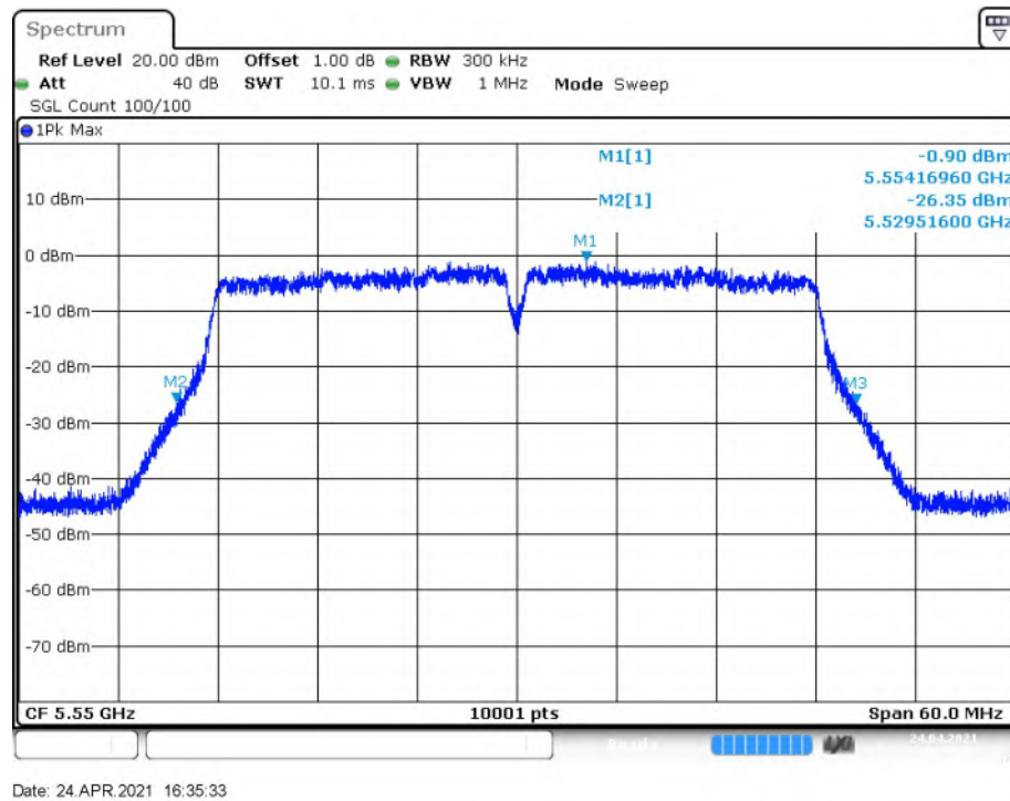
Fig. 15 Occupied 26dB Bandwidth (802.11n-HT40, 5550MHz)
