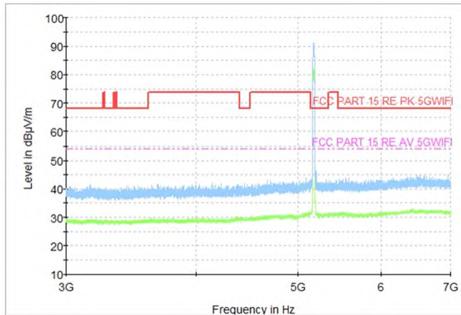
Fig. 95 Transmitter Spurious Emission (All channel, 3GHz~7GHz)
