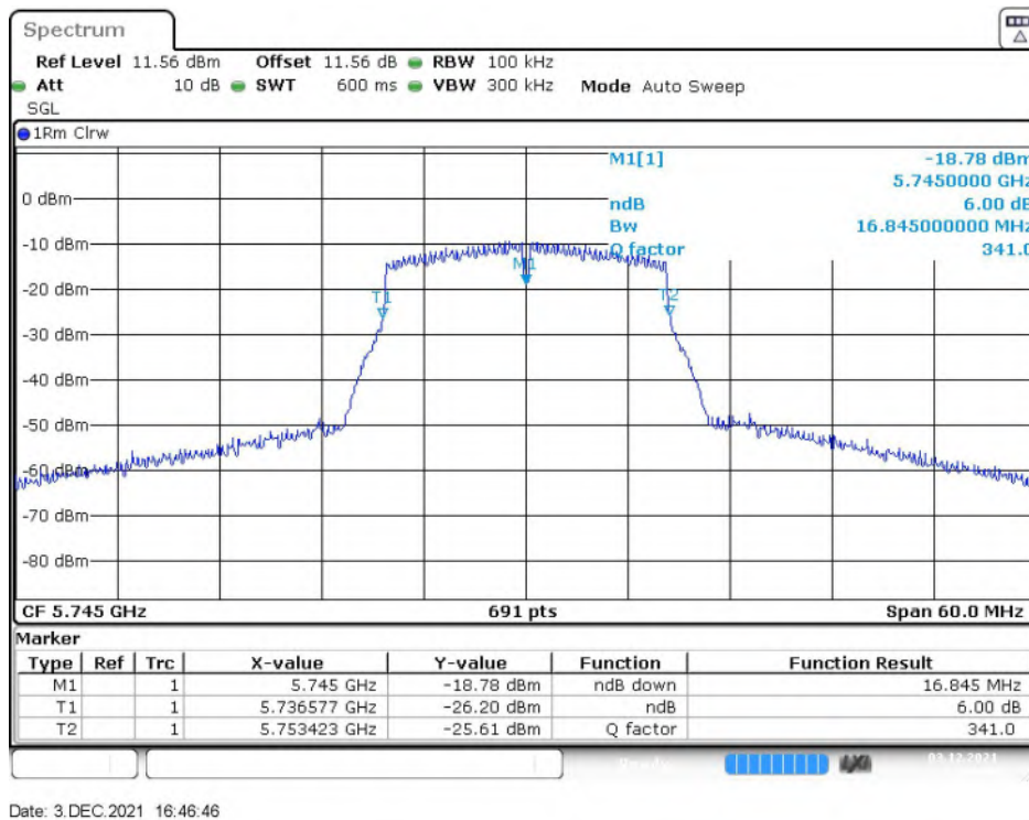
Fig. 21 Occupied 6dB Bandwidth (802.11a, 5745MHz)
