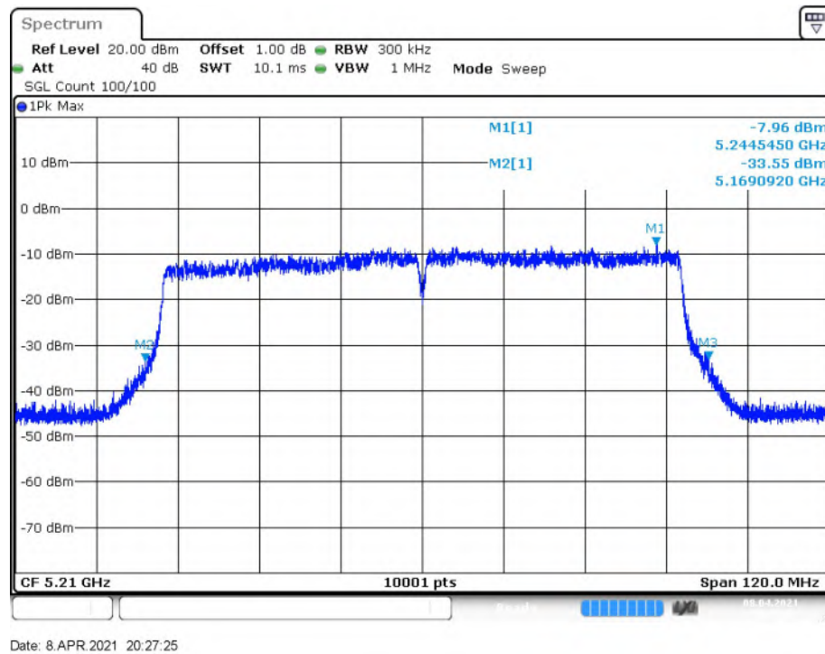
Fig. 17 Occupied 26dB Bandwidth (802.11ac-VHT80, 5210MHz)
