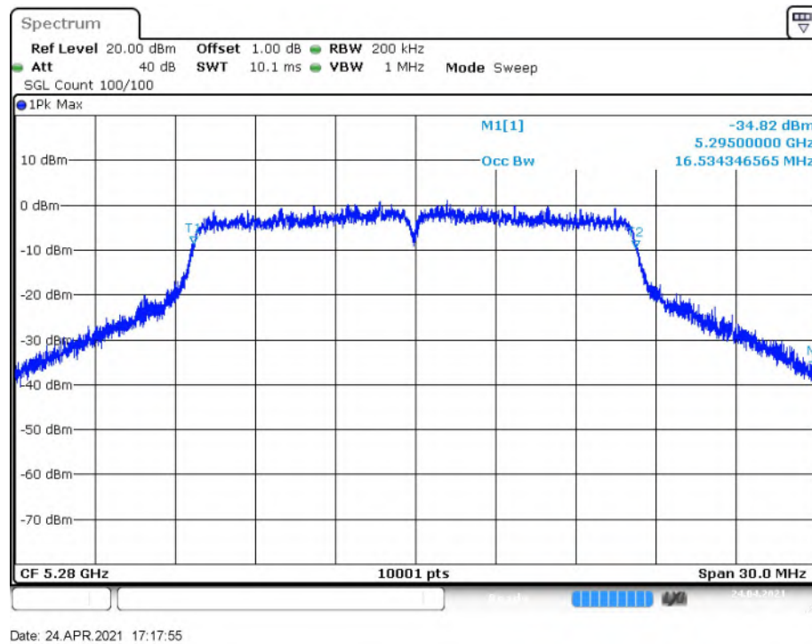
Fig. 5 Occupied 26dB Bandwidth (802.11a, 5280MHz)
