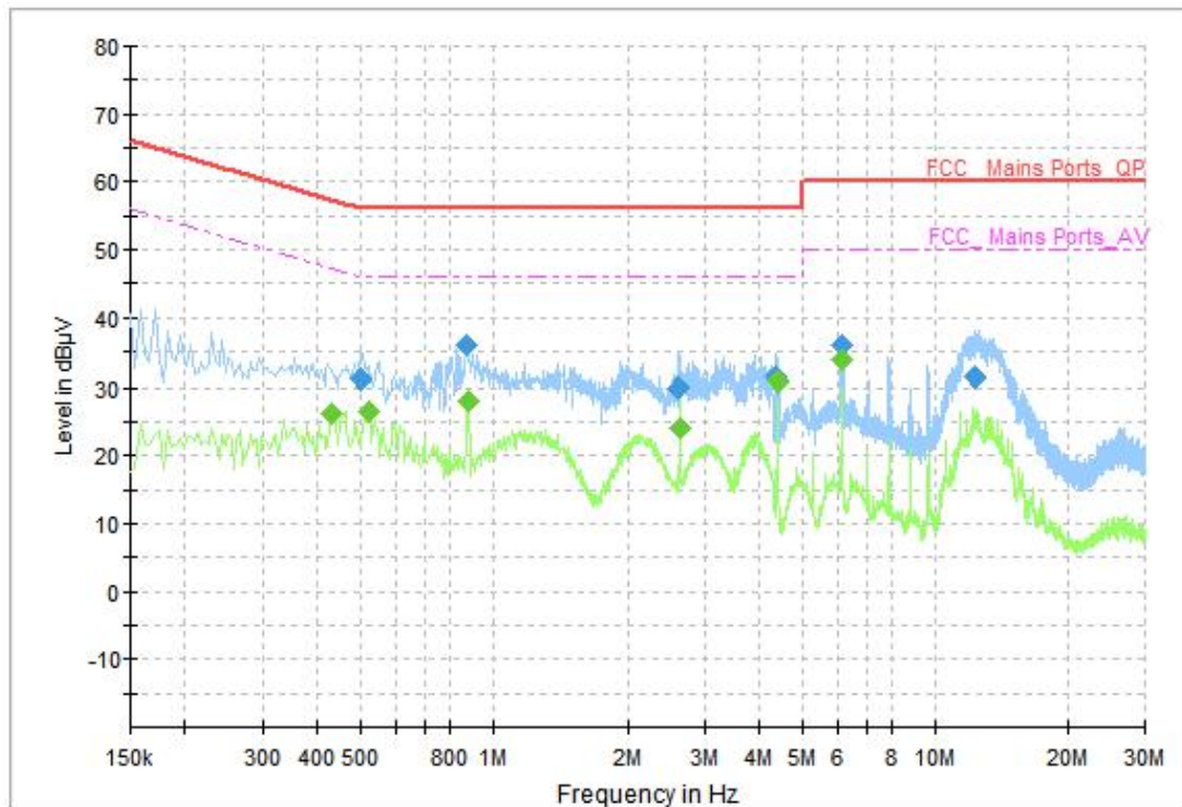
Fig. 99 AC Power line Conducted Emission (Traffic)
