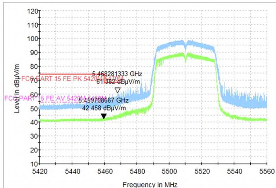
Fig. 59 Band Edges (802.11n-HT40, CH102 5510MHz)
