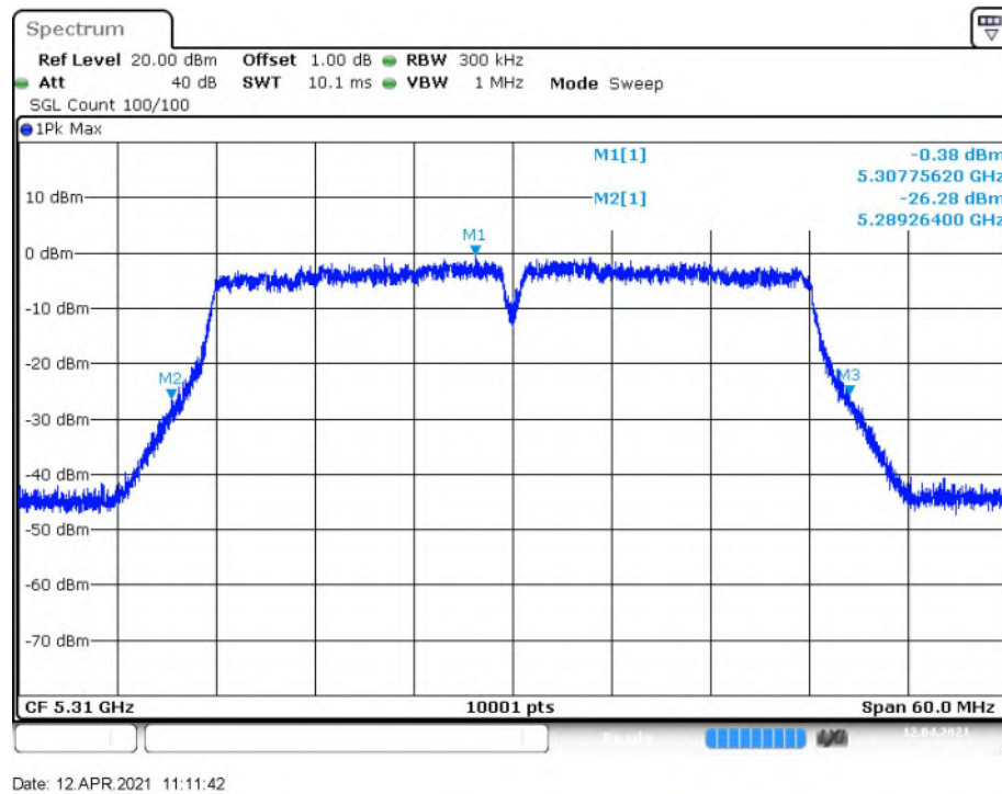
Fig. 13 Occupied 26dB Bandwidth (802.11n-HT40, 5310MHz)
