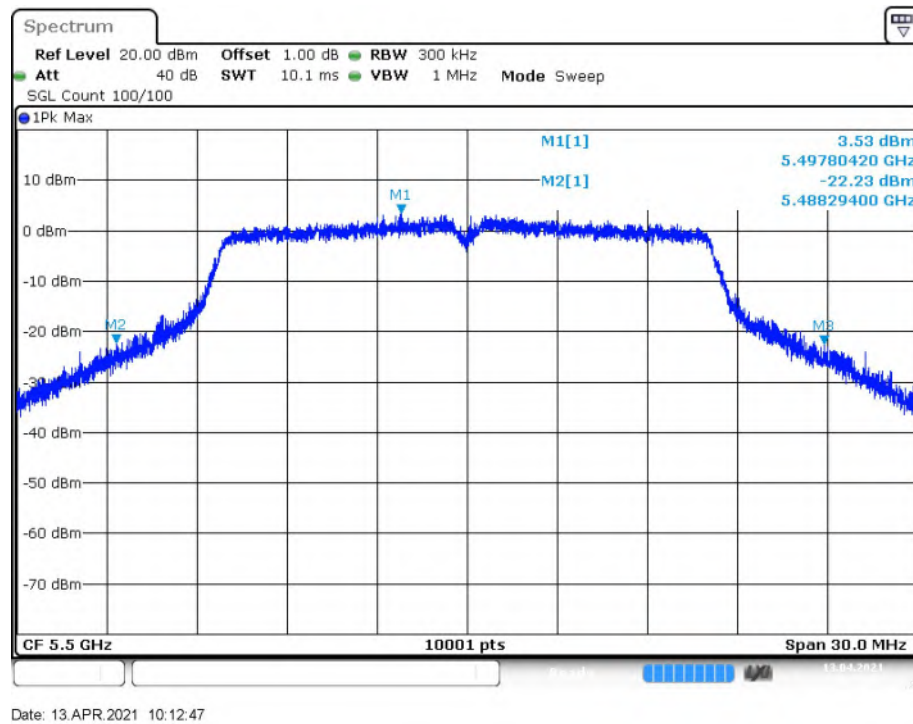
Fig. 7 Occupied 26dB Bandwidth (802.11a, 5500MHz)
