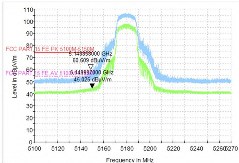
Fig. 51 Band Edges (802.11a, CH36 5180MHz)
