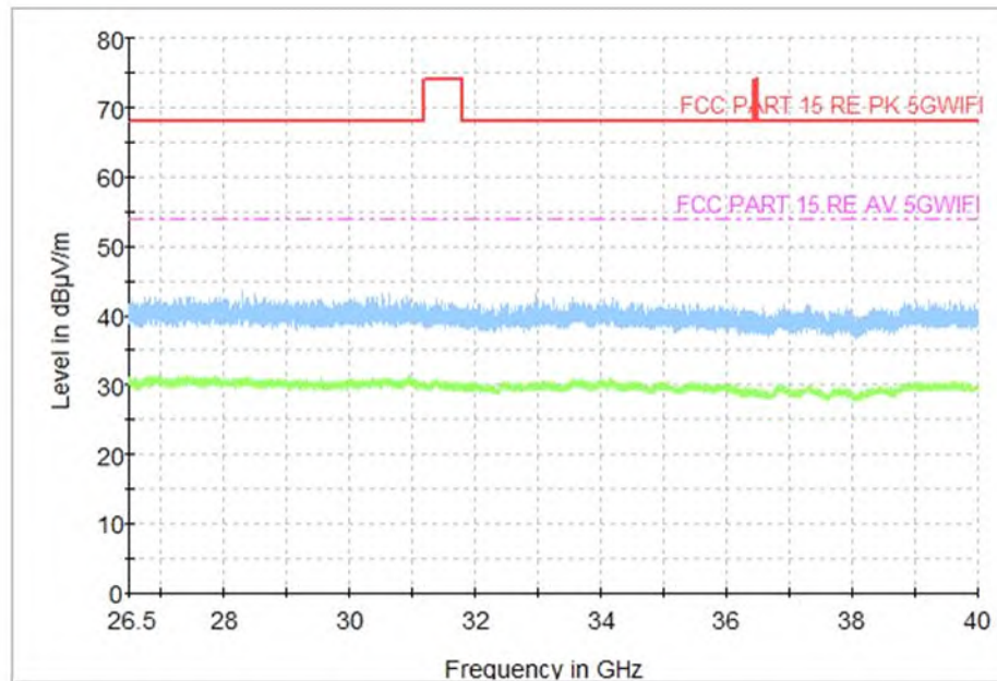
Fig. 97 Transmitter Spurious Emission (All channel, 26.5GHz~40GHz)
