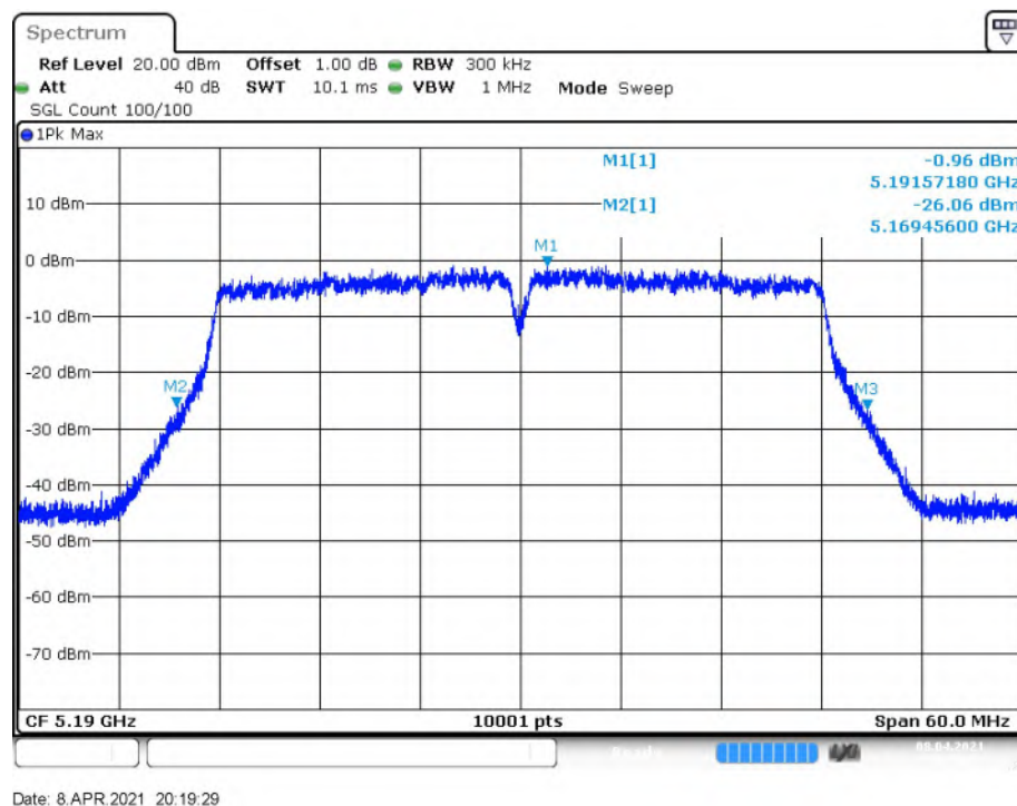
Fig. 10 Occupied 26dB Bandwidth (802.11n-HT40, 5190MHz)
