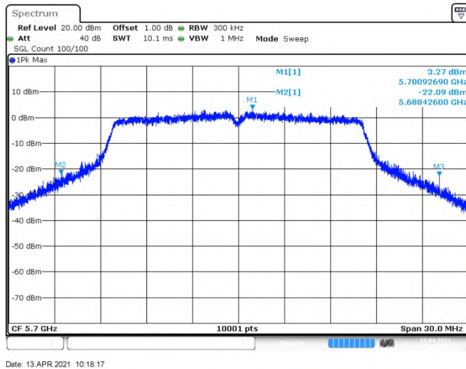
Fig. 9 Occupied 26dB Bandwidth (802.11a, 5700MHz)
