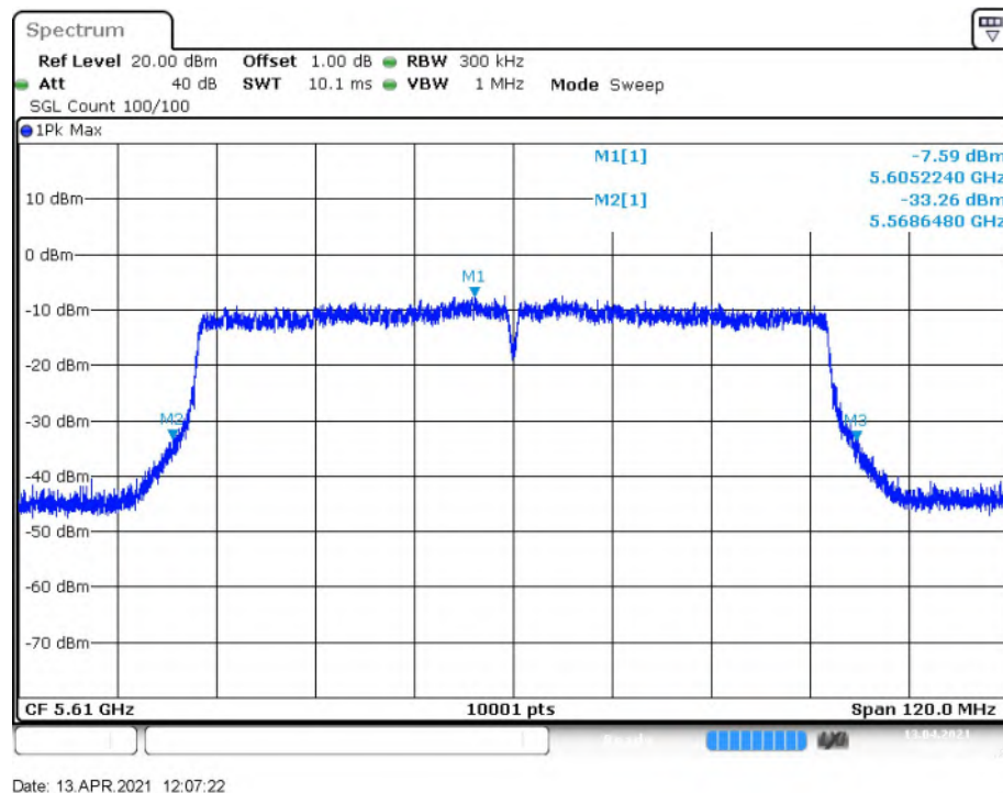
Fig. 20 Occupied 26dB Bandwidth (802.11ac-VHT80, 5610MHz)
