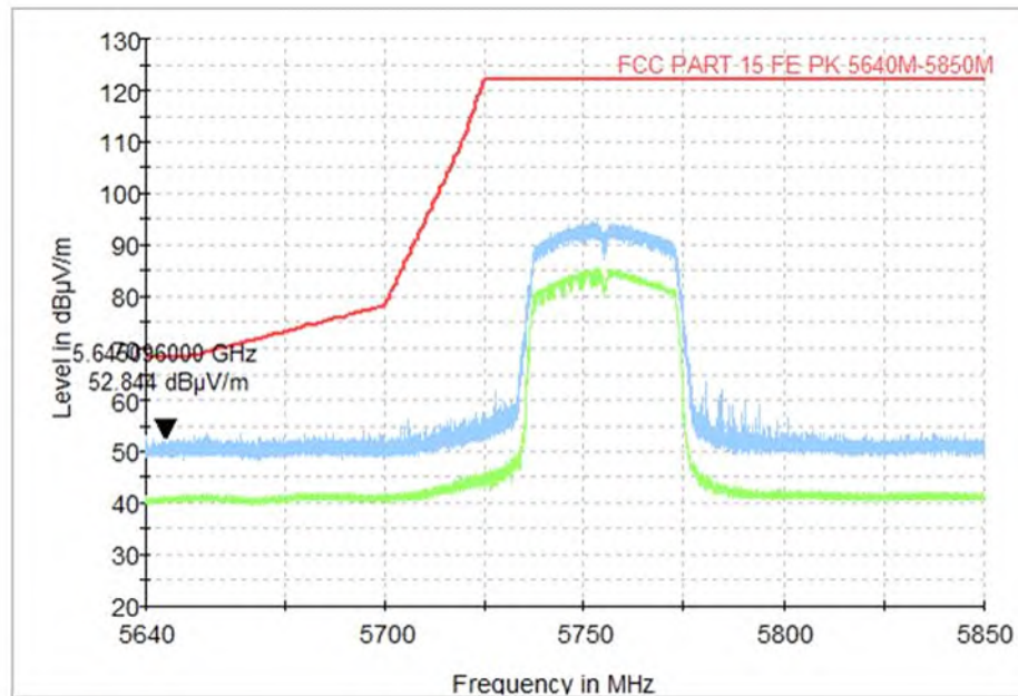
Fig. 61 Band Edges (802.11n-HT40, CH151 5755MHz)
