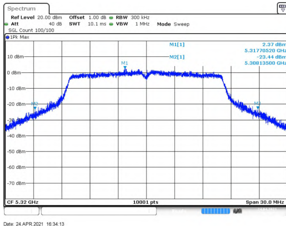
Fig. 6 Occupied 26dB Bandwidth (802.11a, 5320MHz)
