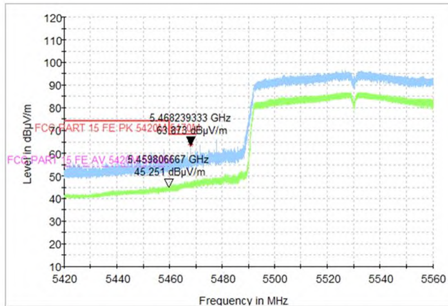
Fig. 65 Band Edges (802.11ac-VHT80, CH106 5530MHz)
