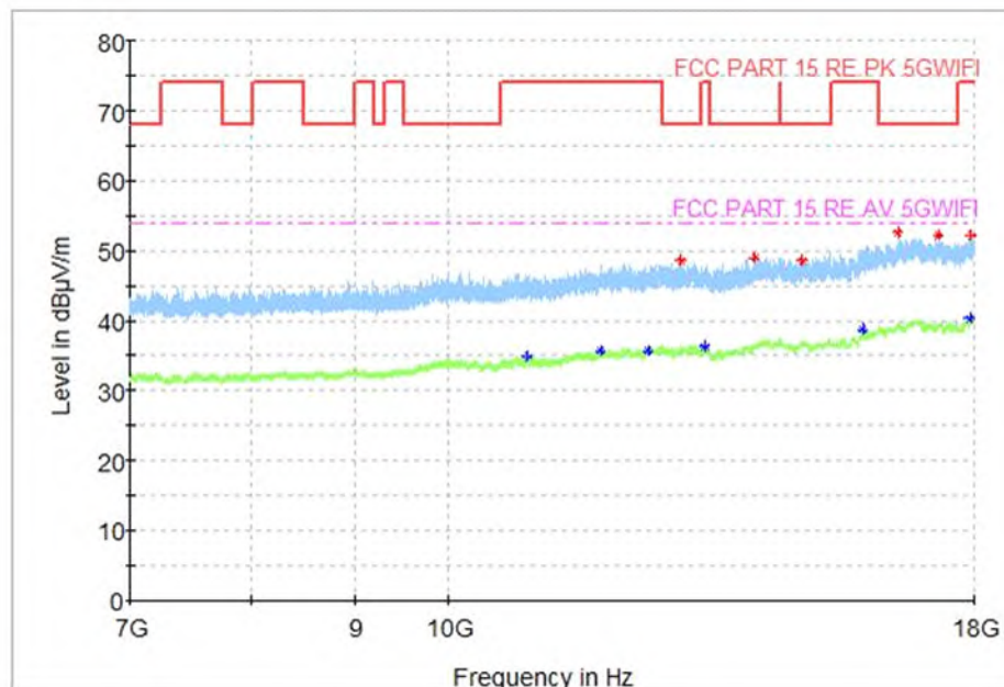
Fig. 68 Transmitter Spurious Emission (802.11a, CH40 5200MHz, 7 GHz-18 GHz)
