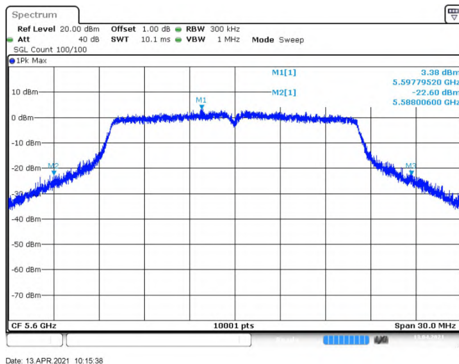
Fig. 8 Occupied 26dB Bandwidth (802.11a, 5600MHz)
