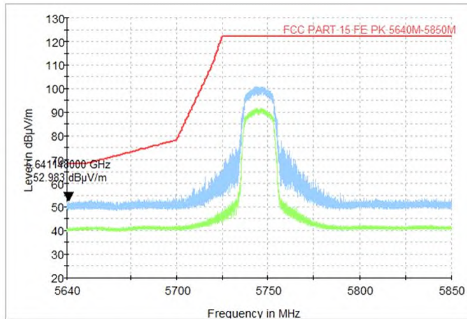
Fig. 55 Band Edges (802.11a, CH149 5745MHz)
