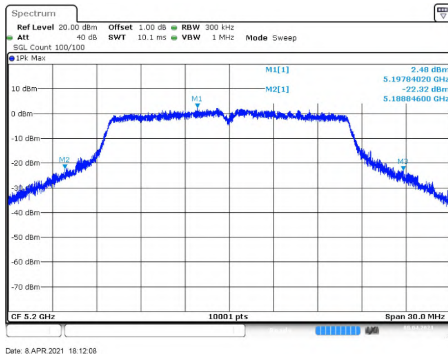
Fig. 2 Occupied 26dB Bandwidth (802.11a, 5200MHz)
