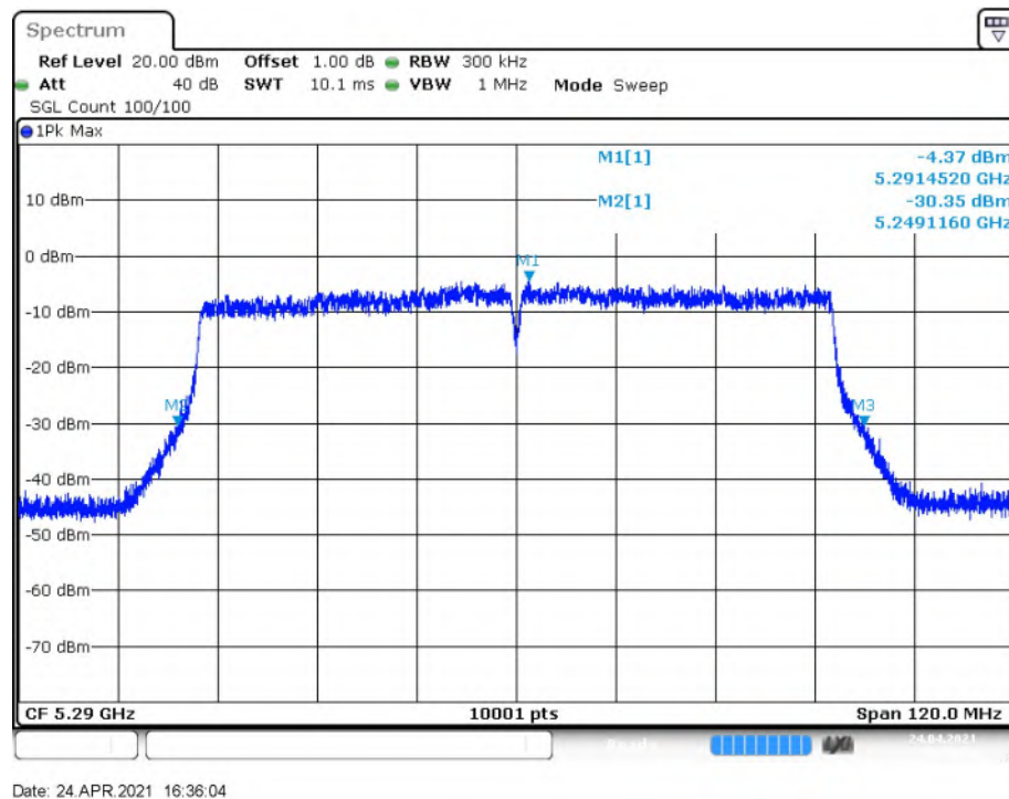
Fig. 18 Occupied 26dB Bandwidth (802.11ac-VHT80, 5290MHz)
