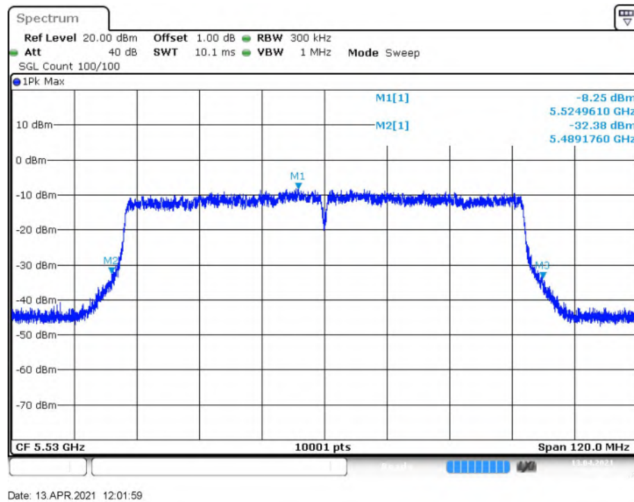
Fig. 19 Occupied 26dB Bandwidth (802.11ac-VHT80, 5530MHz)
