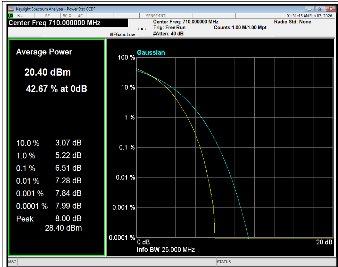
Band17 64QAM BW=10MHz Channel=23790 RB Size=50 Position=#0
