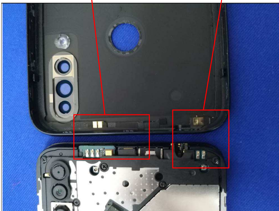
Diversity Antenna
