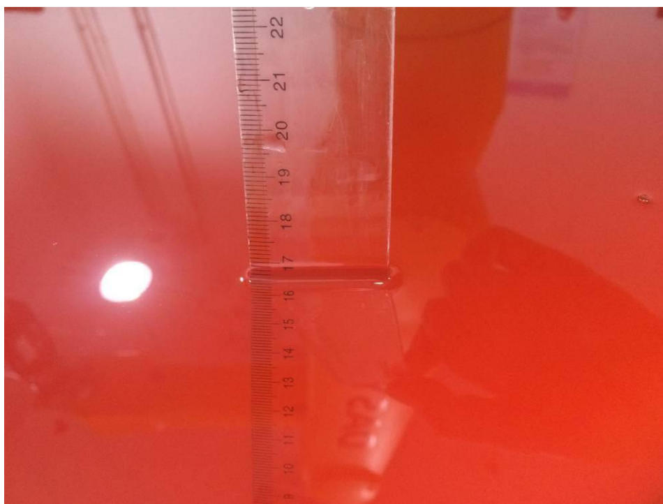
Picture 9-6: Liquid depth in the Flat Phantom (1900 MHz Body)
