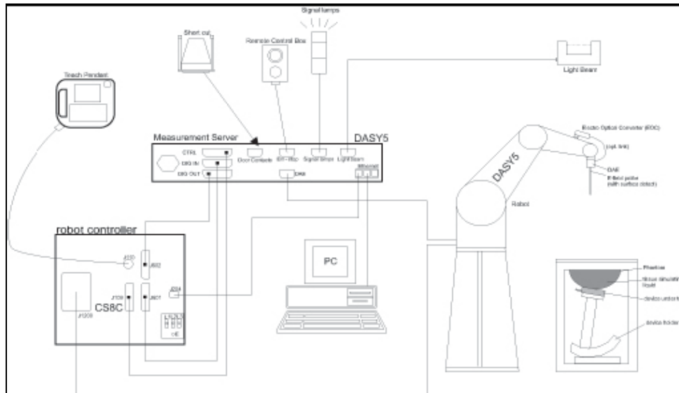
● A standard high precision 6-axis robot (Stäubli TX=RX family) with controller, teach pendant and software. An arm extension for accommodating the data acquisition electronics (DAE). ● An isotropic field probe optimized and calibrated for the targeted measurement. ● A data acquisition electronics (DAE) which performs the signal amplification, signal multiplexing, AD-conversion, offset measurements, mechanical surface detection, collision detection, etc. The unit is battery powered with standard or rechargeable batteries. The signal is optically transmitted to the EOC. ● The Electro-optical converter (EOC) performs the conversion from optical to electrical signals for the digital communication to the DAE. To use optical surface detection, a special version of the EOC is required. The EOC signal is transmitted to the measurement server. ● The function of the measurement server is to perform the time critical tasks such as signal filtering, control of the robot operation and fast movement interrupts. ● The Light Beam used is for probe alignment. This improves the (absolute) accuracy of the probe positioning. ● A computer running WinXP and the DASY5 software. ● Remote control and teach pendant as well as additional circuitry for robot safety such as warning lamps, etc. ● The phantom, the device holder and other accessories according to the targeted measurement.
