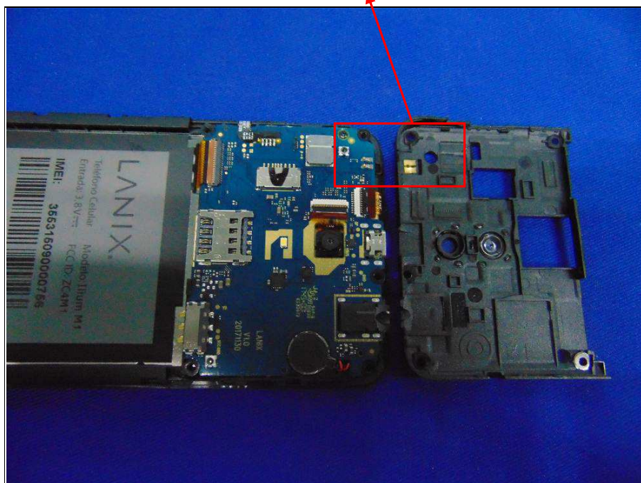
BT/WLAN/GPS Antenna
