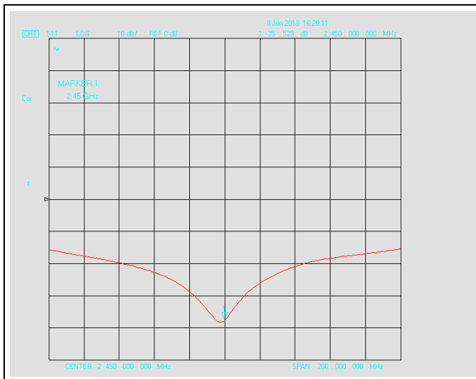
Dipole Verification plot: SID 2450 2450MHz for Head:
