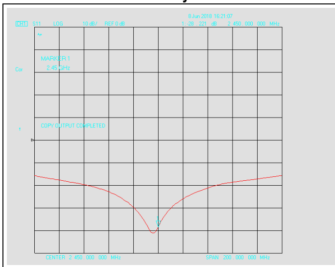
Dipole Verification plot: SID 2450 2450MHz for Body:
