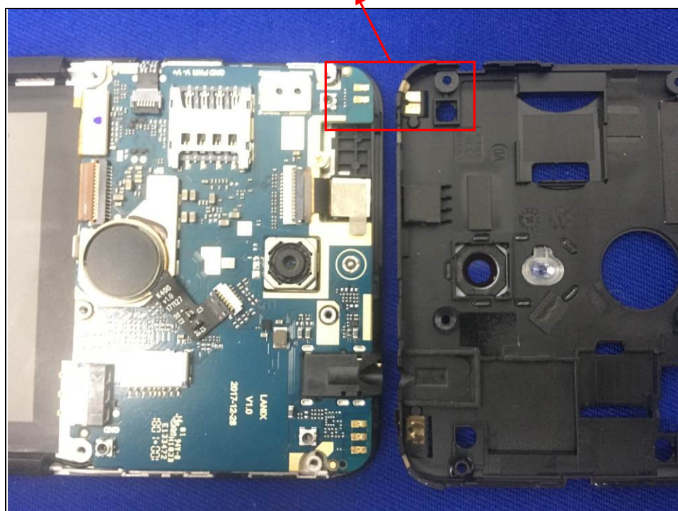
BT/WLAN Antenna
