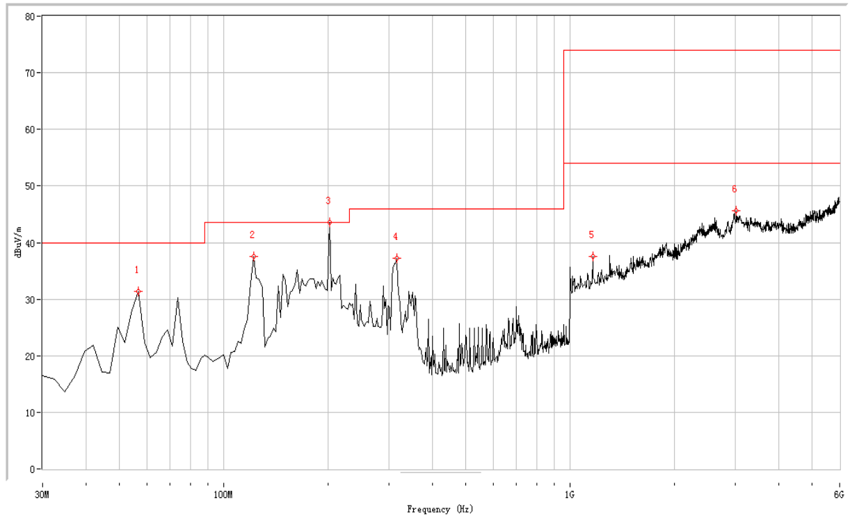
(Plot C: Test Antenna Horizontal 30M - 6G)
