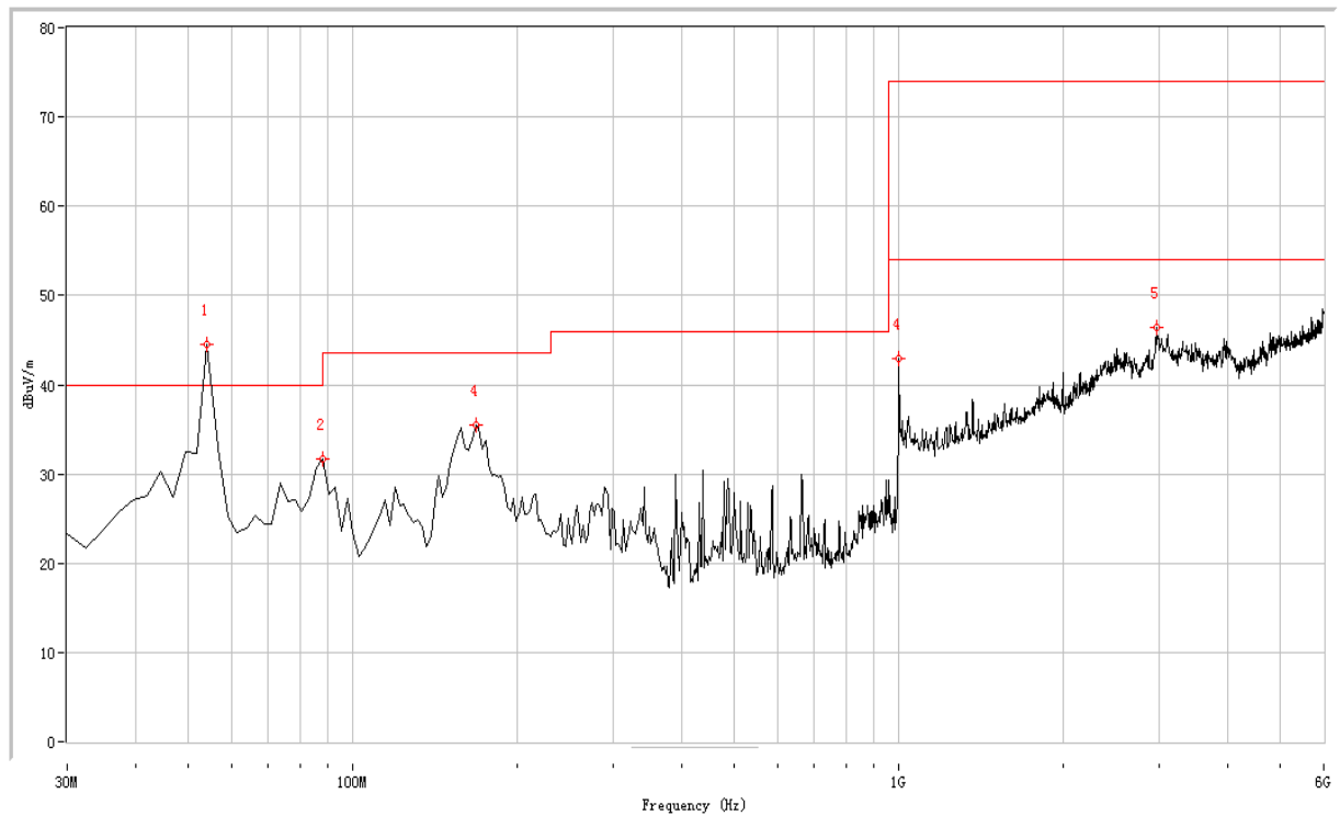
(Plot B: Test Antenna Vertical 30M - 6G)
