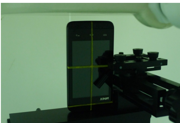
Bottom Side, Test Separation 1 cm
