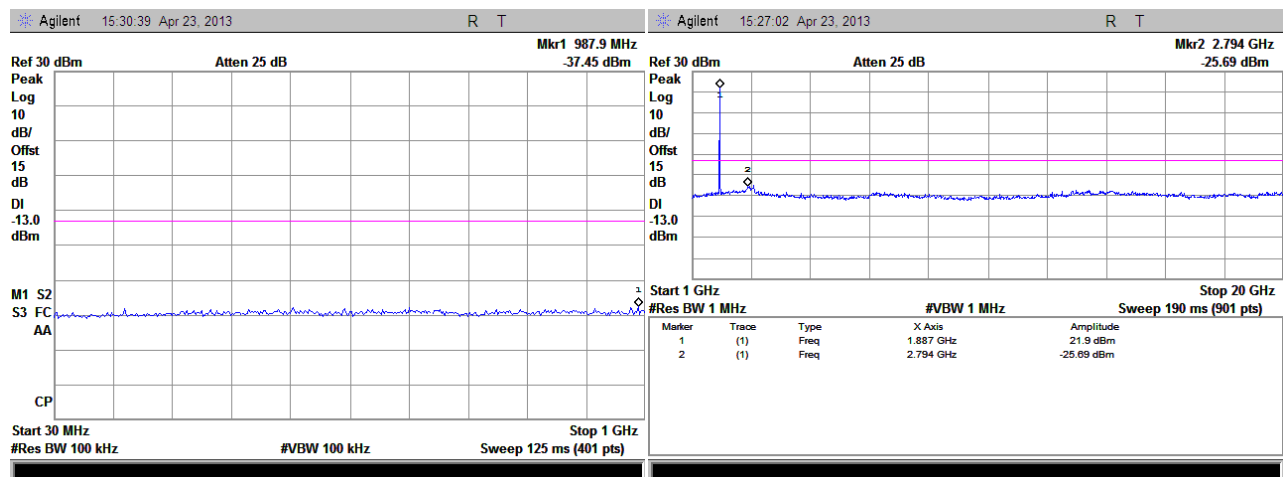
(Plot F2: WCDMA1900MHz Channel = 9400, 30MHz to 20GHz)
