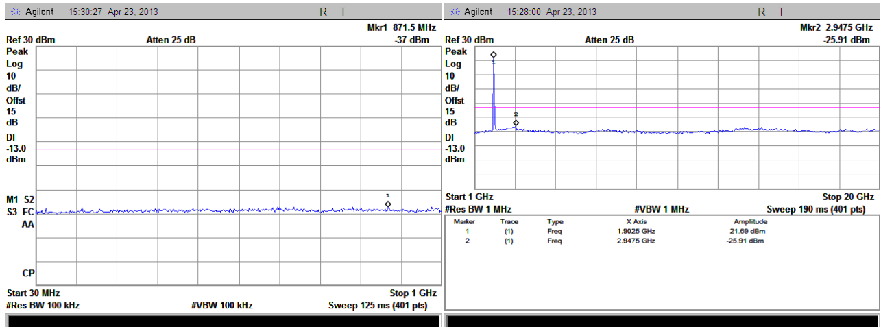
(Plot F3: WCDMA1900MHz Channel = 9538, 30MHz to 20GHz)
