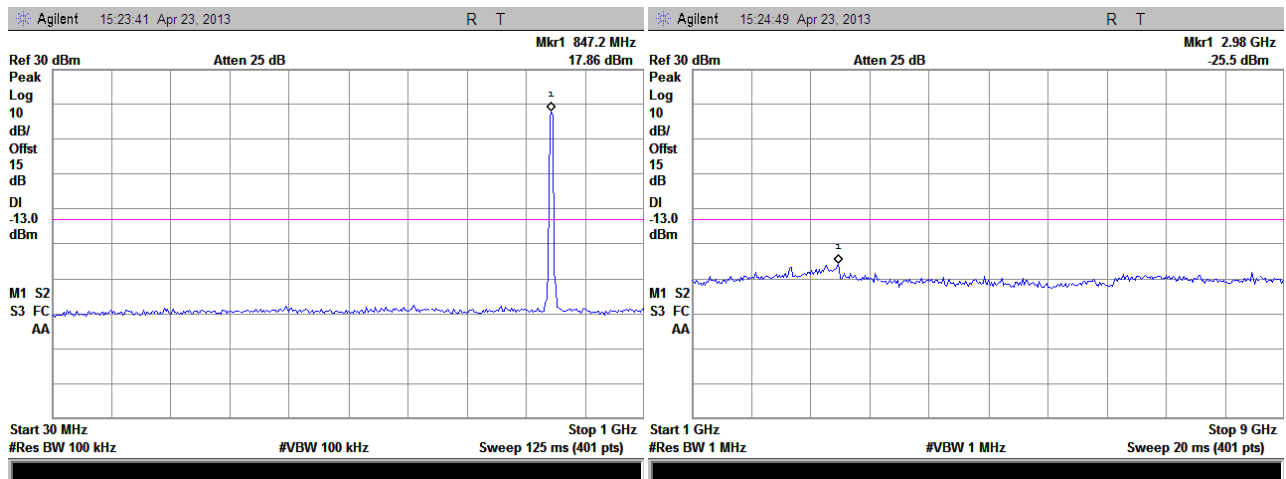
(Plot E3: WCDMA850MHz Channel = 4233, 30MHz to 9GHz)
