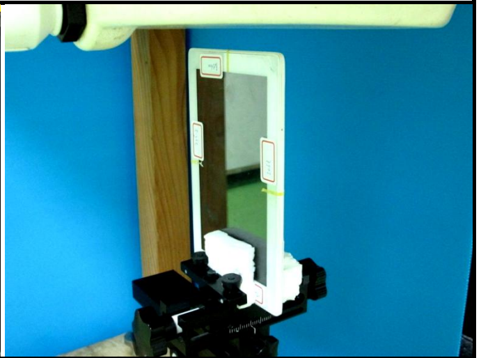
Bottom Side of EUT with 1.8 cm Gap
