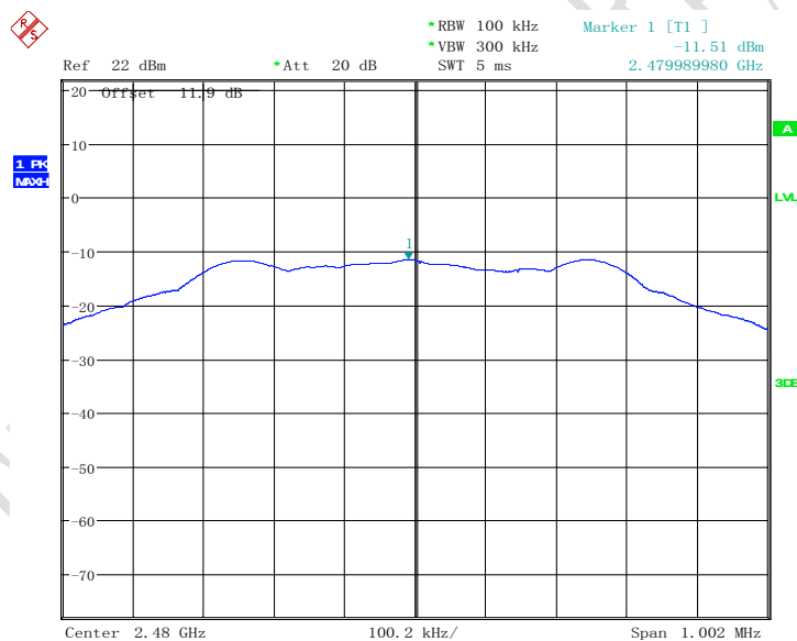
Fig.5 Power spectral density: CH19 PSD/100KHz
