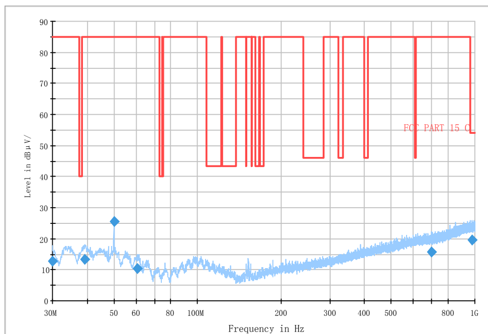
Fig.21 Radiated emission Ch19, 30MHz-1GHz
