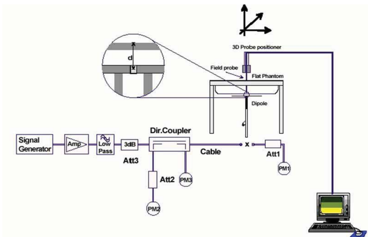
System Check Set-up
