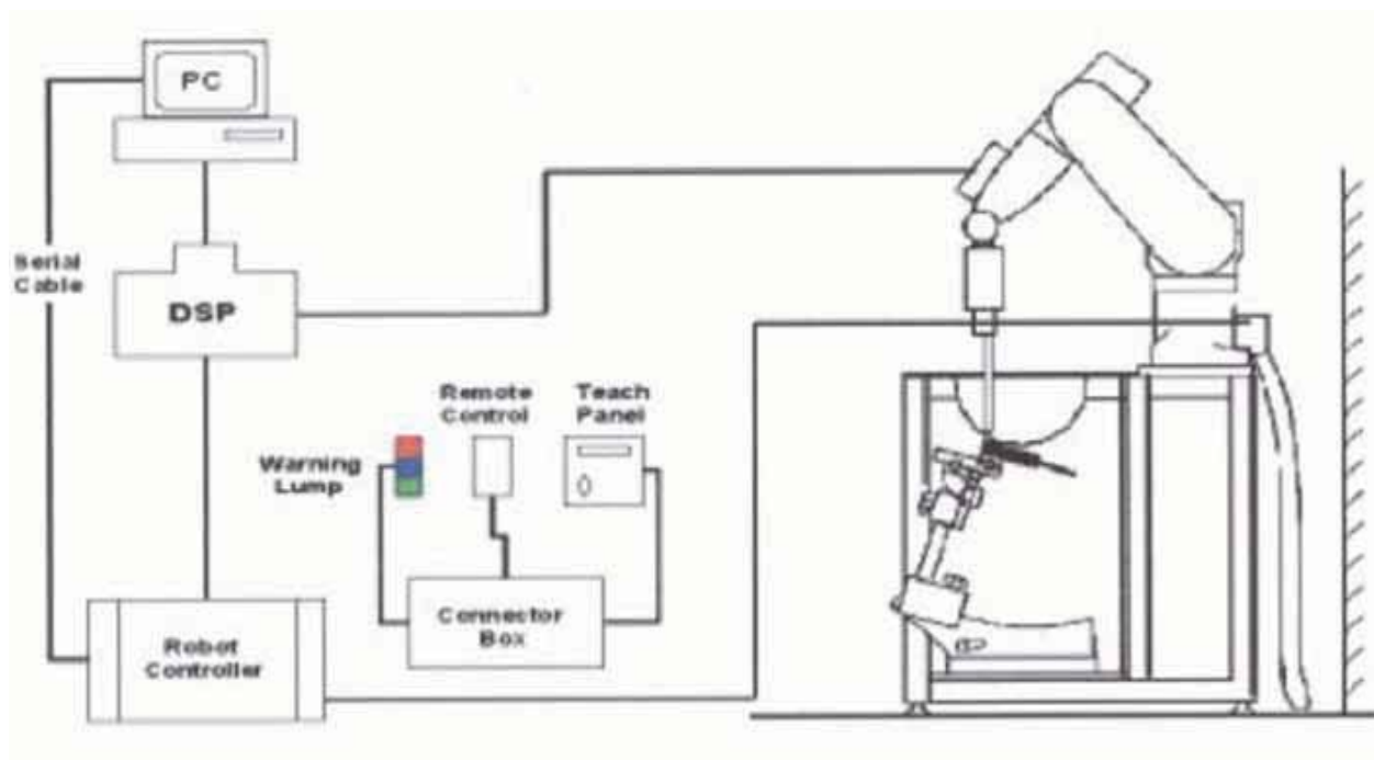
Figure 6.1 SAR Lab Test Measurement Set-up
