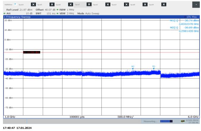
Figure 7.5-36: Conducted spurious emissions 1- 6, high channel, 12.5 kHz, analog, FCC part 22 & 74
