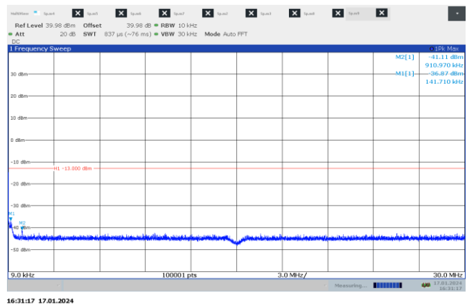
Figure 7.5-22: Conducted spurious emissions 9k- 30 MHz, low channel, 12.5 kHz, analog, FCC part 22 & 74
