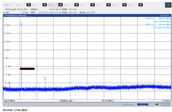
Figure 7.5-58: Conducted spurious emissions 0.03- 1 GHz, low channel, 25 kHz, analog, FCC part 90, 22 & 74, RSS 119
