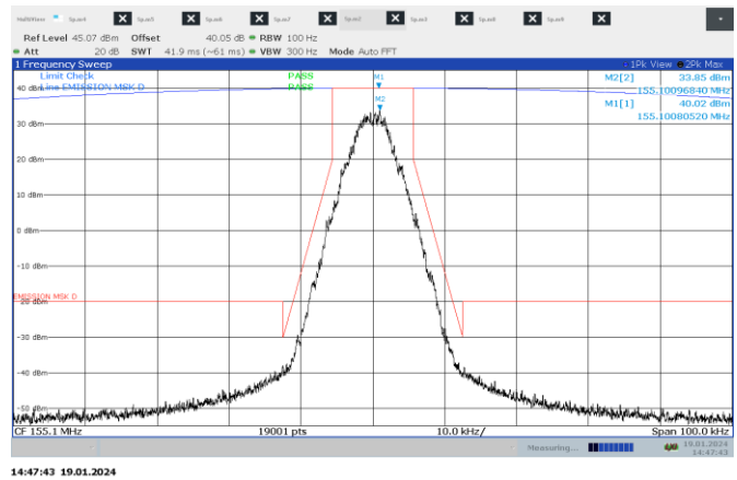
Figure 7.5-8: Emission mask D for mid channel, 12.5 kHz digital
