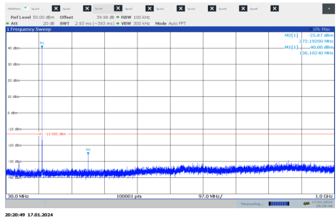
Figure 7.5-46: Conducted spurious emissions 0.03- 1 GHz, low channel, 12.5 kHz, digital, FCC part 22 & 74
