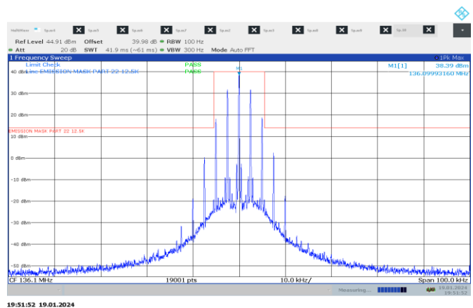
Figure 7.5-10: Emission mask FCC part 22 for low channel, 12.5 kHz analog
