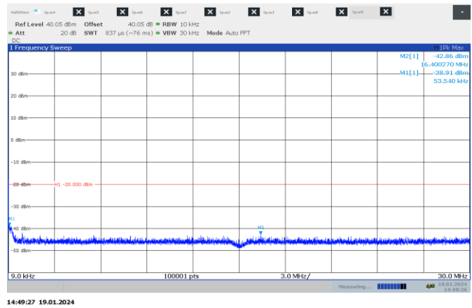
Figure 7.5-38: Conducted spurious emissions 9k 30 MHz, mid channel, 12.5 kHz, digital, FCC part 90, RSS 119
