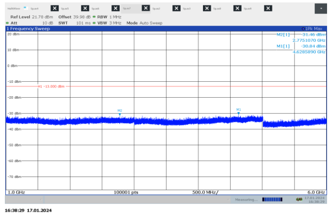
Figure 7.5-34: Conducted spurious emissions 1- 6, low channel, 12.5 kHz, analog, FCC part 22 & 74
