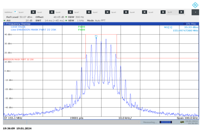
Figure 7.5-14: Emission mask FCC part 22 for low channel, 25 kHz analog
