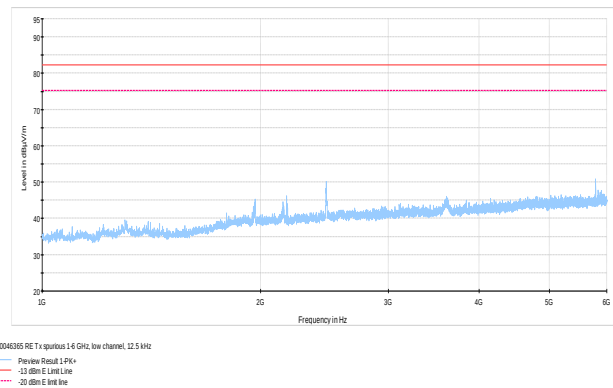
Figure 7.5-67: Radiated spurious emissions 1-6 GHz, low channel, 12.5 kHz, analog
