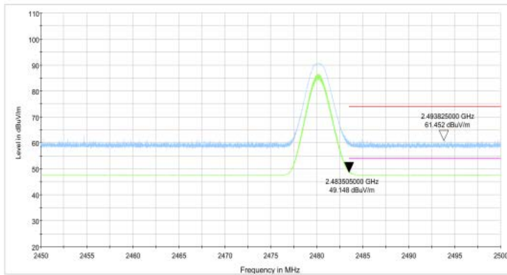
Fig.2. Frequency Band Edges: GFSK, 2480 MHz, 2.45 GHz - 2.50GHz
