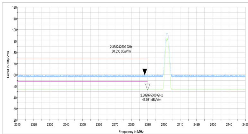
Fig.3. Frequency Band Edges: GFSK, 2402 MHz, 2.31 GHz - 2.45GHz
