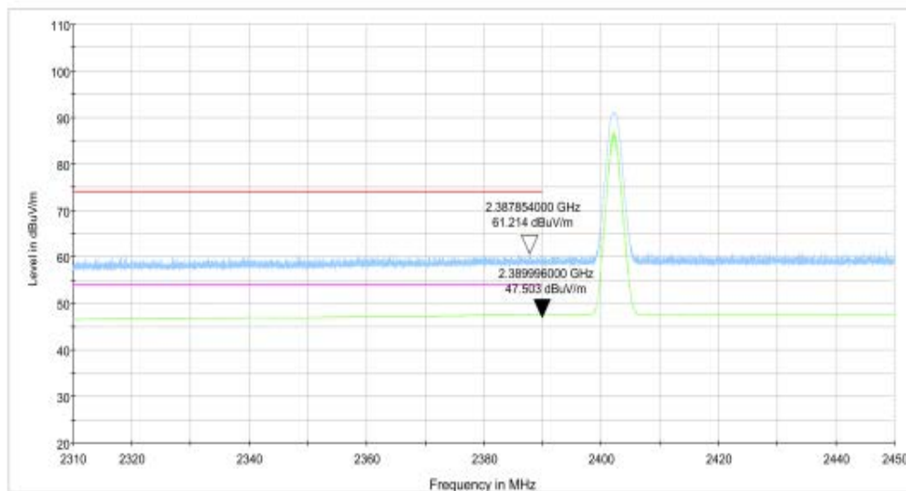
Fig.1. Frequency Band Edges: GFSK, 2402 MHz, 2.31 GHz – 2.45GHz
