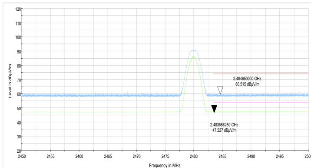
Fig.4. Frequency Band Edges: GFSK, 2480 MHz, 2.45 GHz - 2.50GHz
