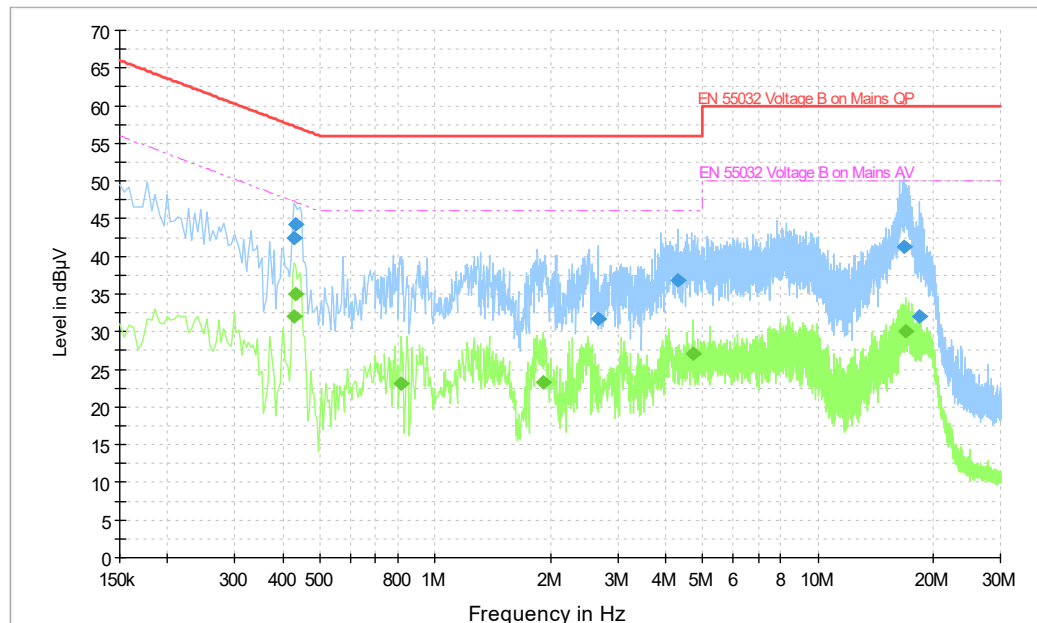
Fig.A.9.1 AC Powerline Conducted Emission- bluetooth
