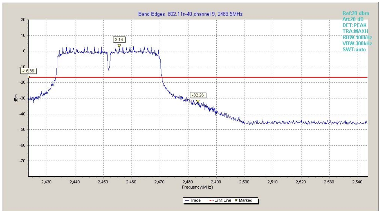
Fig.A.5.2 Band Edges (802.11n-HT40, Ch 9)
