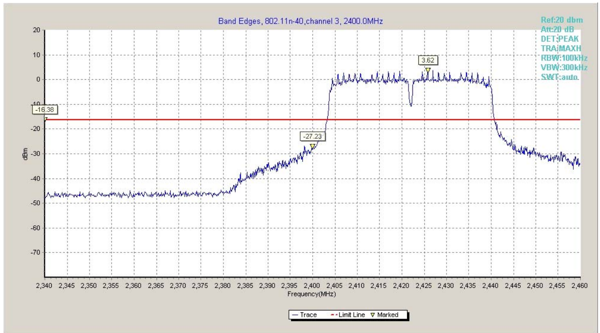
Fig.A.5.1 Band Edges (802.11n-HT40, Ch 3)
