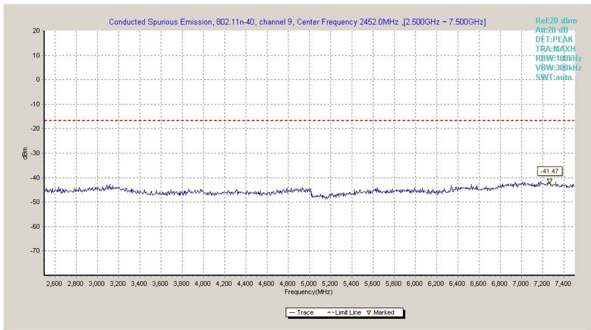
Fig.A.6.1.20 Transmitter Spurious Emission - Conducted (802.11n-HT40, Ch9, 2.5 GHz-7.5 GHz)
