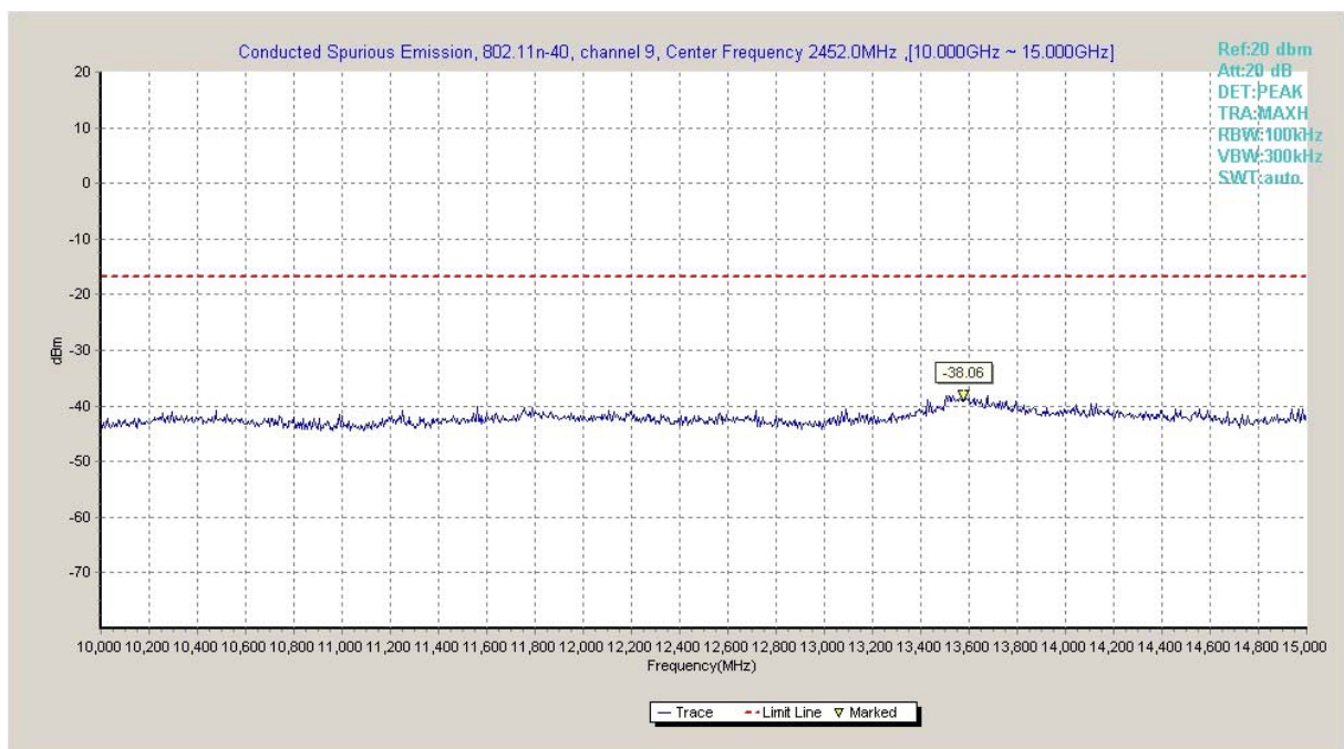
Fig.A.6.1.22 Transmitter Spurious Emission - Conducted (802.11n-HT40, Ch9, 10 GHz-15 GHz)
