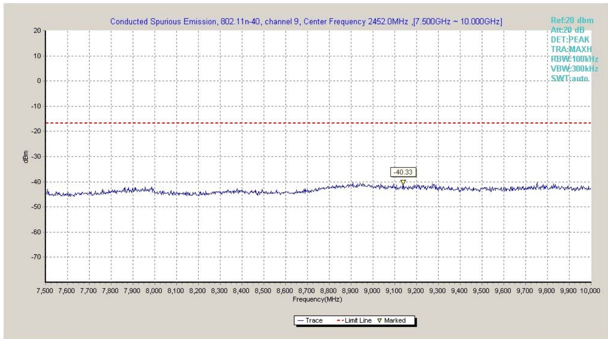
Fig.A.6.1.21 Transmitter Spurious Emission - Conducted (802.11n-HT40, Ch9, 7.5 GHz-10 GHz)
