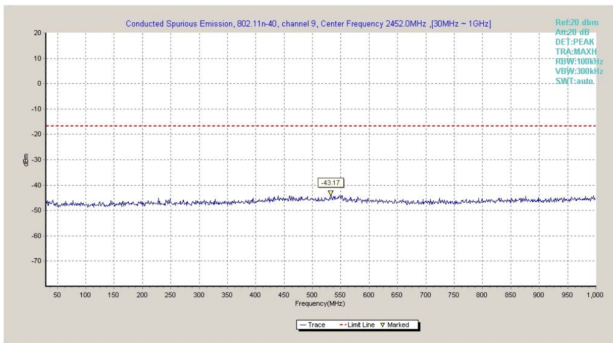
Fig.A.6.1.18 Transmitter Spurious Emission - Conducted (802.11n-HT40, Ch9, 30 MHz-1 GHz)
