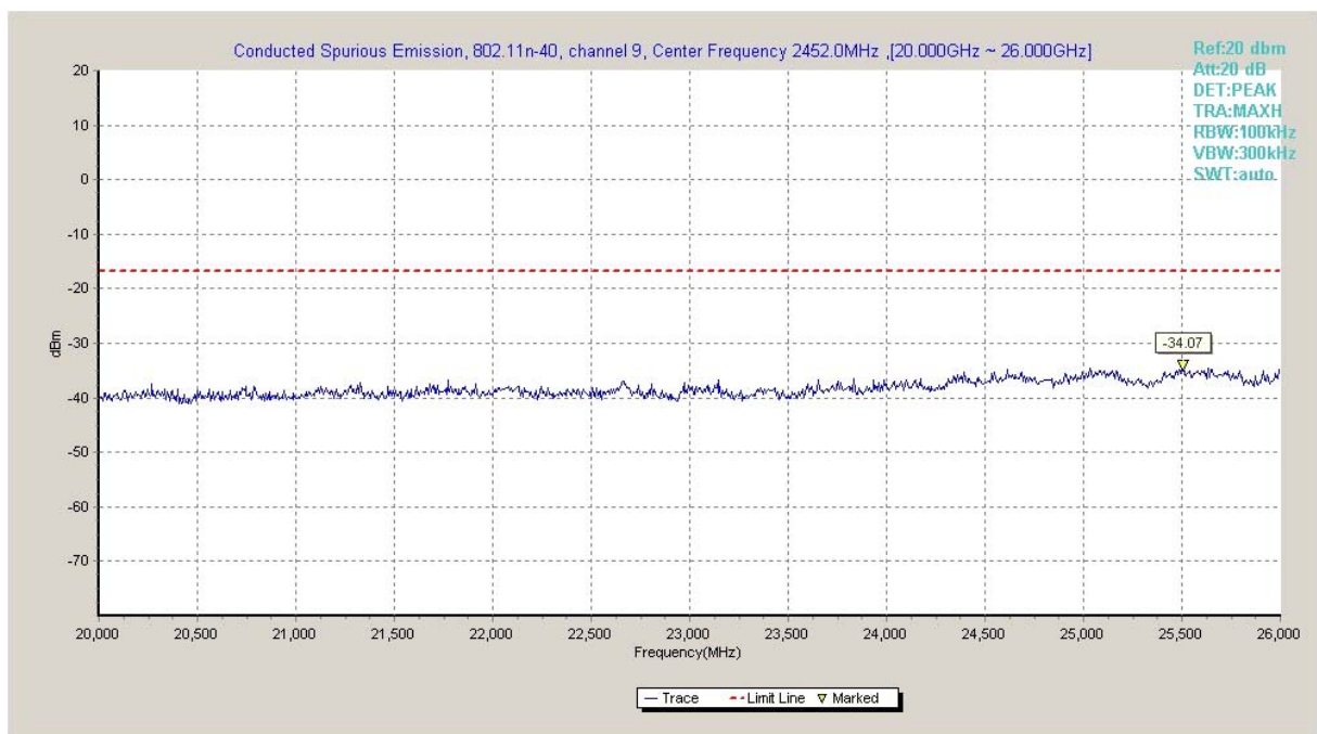
Fig.A.6.1.24 Transmitter Spurious Emission - Conducted (802.11n-HT40, Ch9, 20 GHz-26 GHz)
