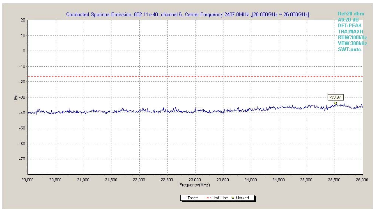
Fig.A.6.1.16 Transmitter Spurious Emission - Conducted (802.11n-HT40, Ch6, 20 GHz-26 GHz)
