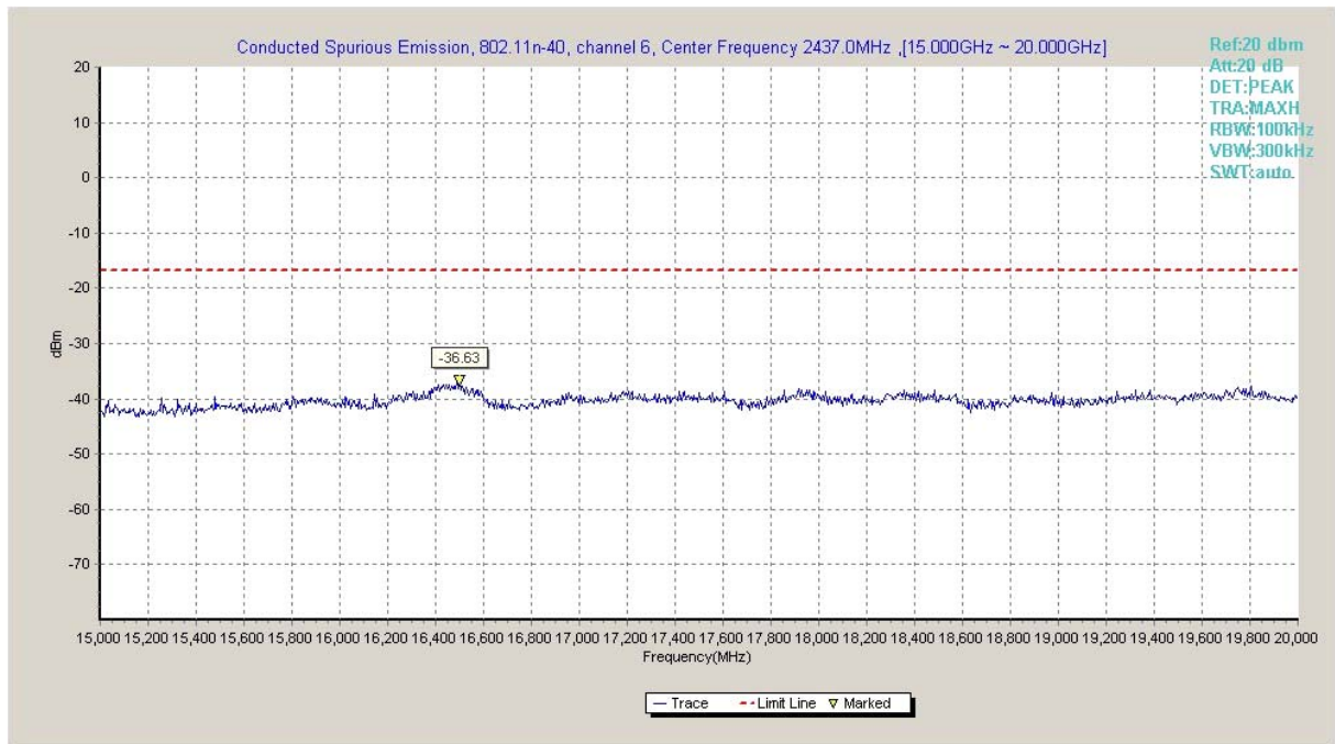
Fig.A.6.1.15 Transmitter Spurious Emission - Conducted (802.11n-HT40, Ch6, 15 GHz-20 GHz)
