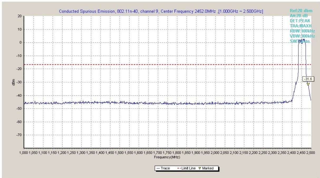
Fig.A.6.1.19 Transmitter Spurious Emission - Conducted (802.11n-HT40, Ch9, 1 GHz-2.5 GHz)
