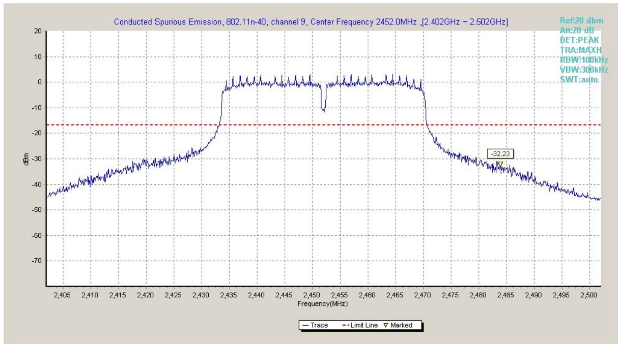
Fig.A.6.1.17 Transmitter Spurious Emission - Conducted (802.11n-HT40, Ch9, Center Frequency)
