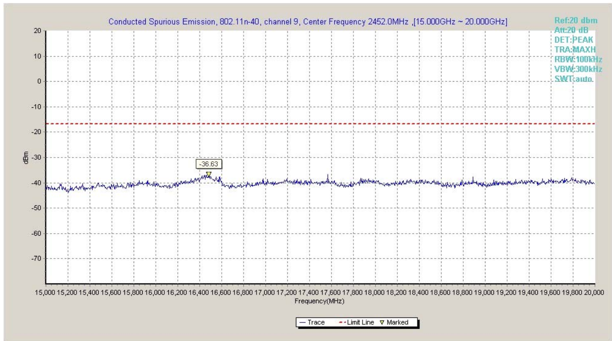
Fig.A.6.1.23 Transmitter Spurious Emission - Conducted (802.11n-HT40, Ch9, 15 GHz-20 GHz)
