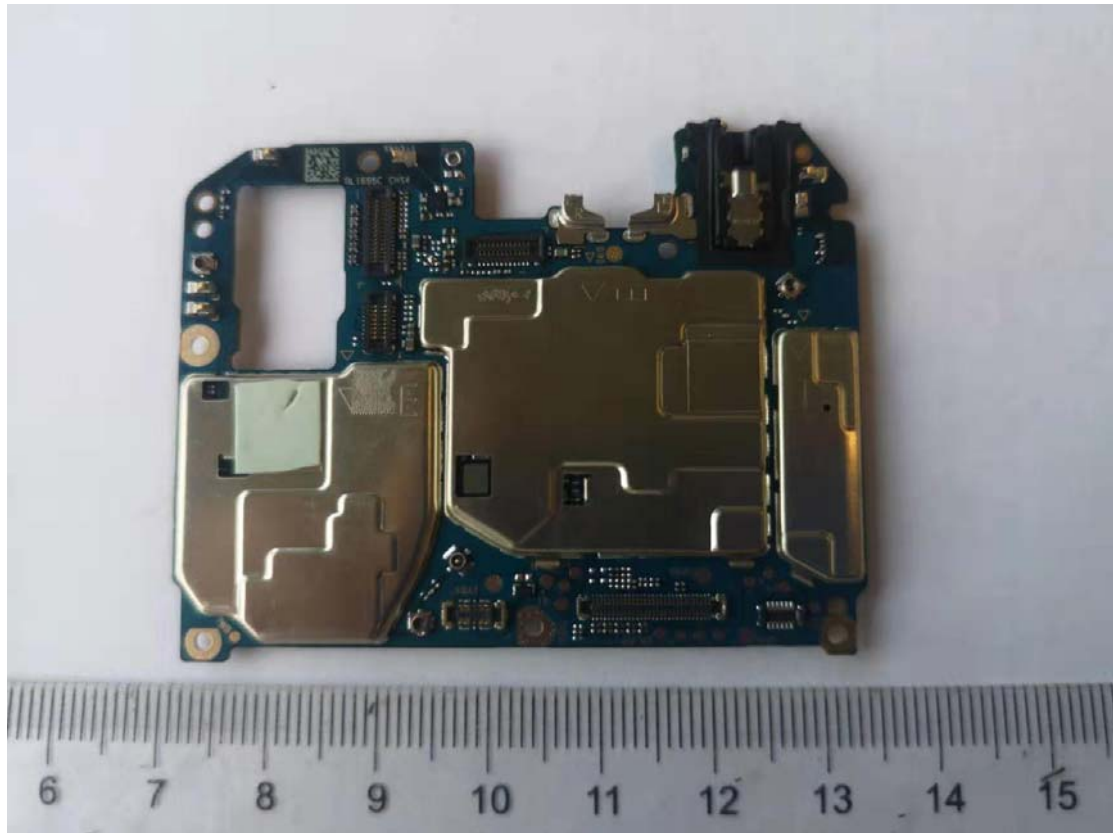
PCB08:
