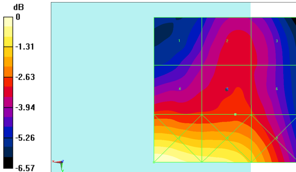
Fig B.3 HAC RF E-Field WiFi2.4G 11g
