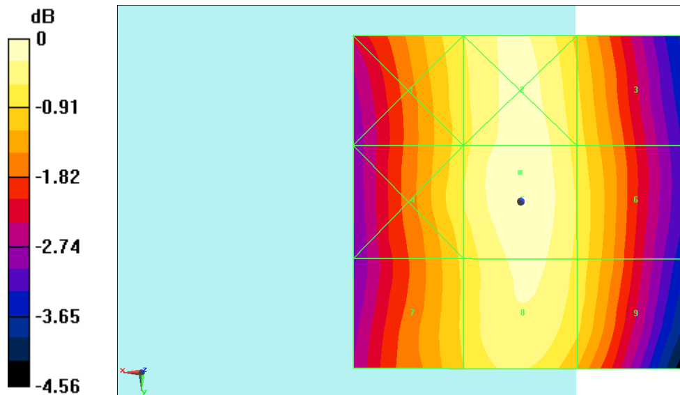
Fig B.1 HAC RF E-Field GSM 850 Low
