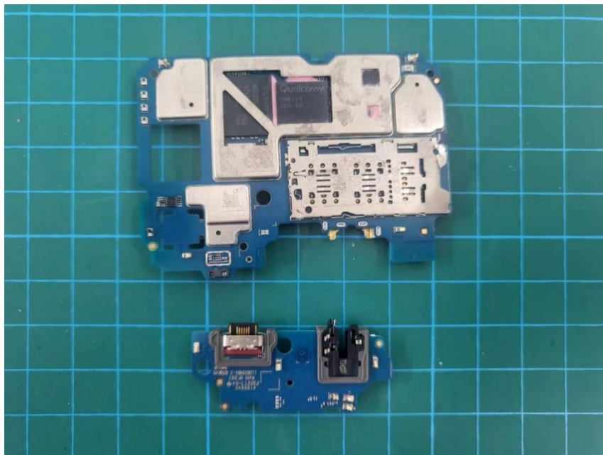
PCB06
