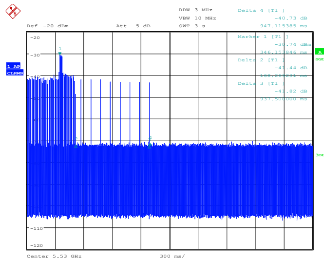
Fig.A.5 channel closing transmission time
