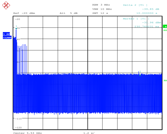
Fig.A.4 Channel move time
