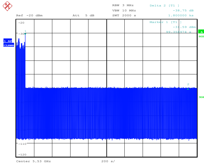
Fig.A.7 Non-Occupancy Period
