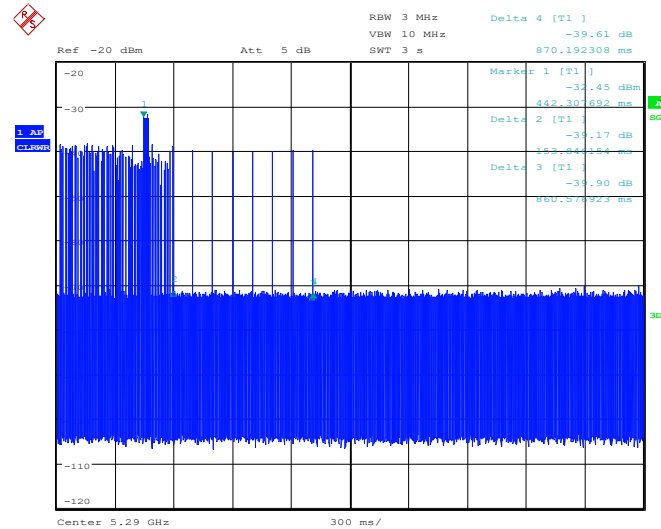
Fig.A.3 channel closing transmission time
