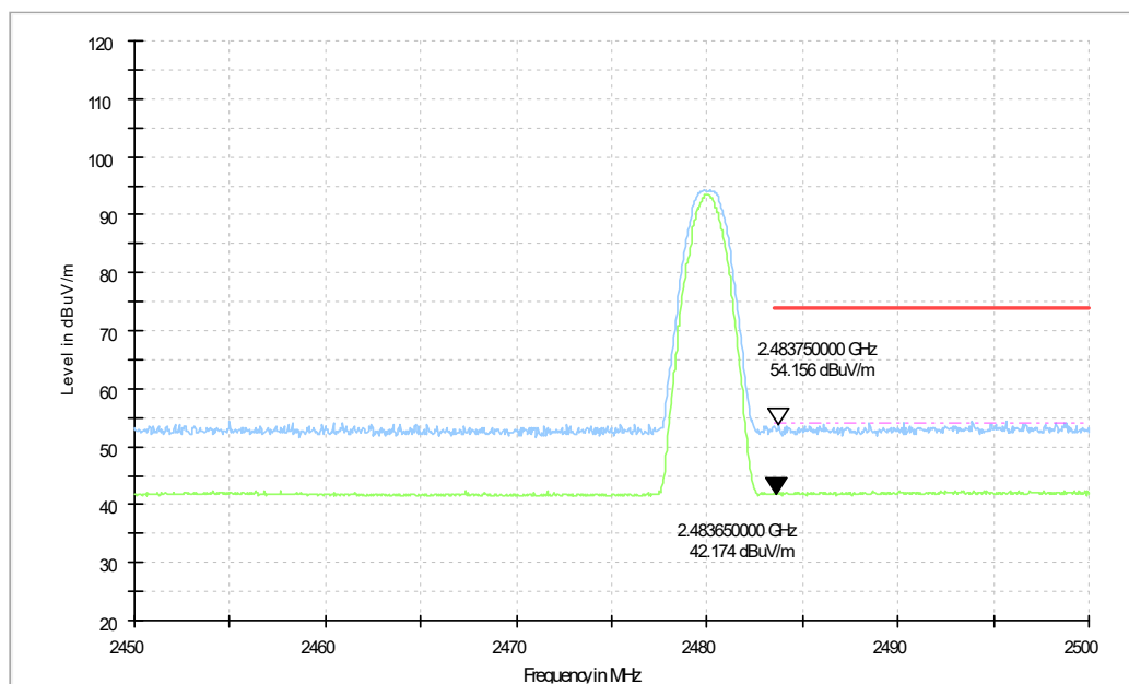
Fig.2. Frequency Band Edges: GFSK, 2480 MHz, Hopping Off, 2.45 GHz - 2.50GHz
