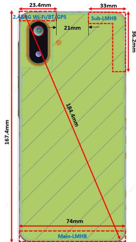
Picture 19 Antenna Locations
