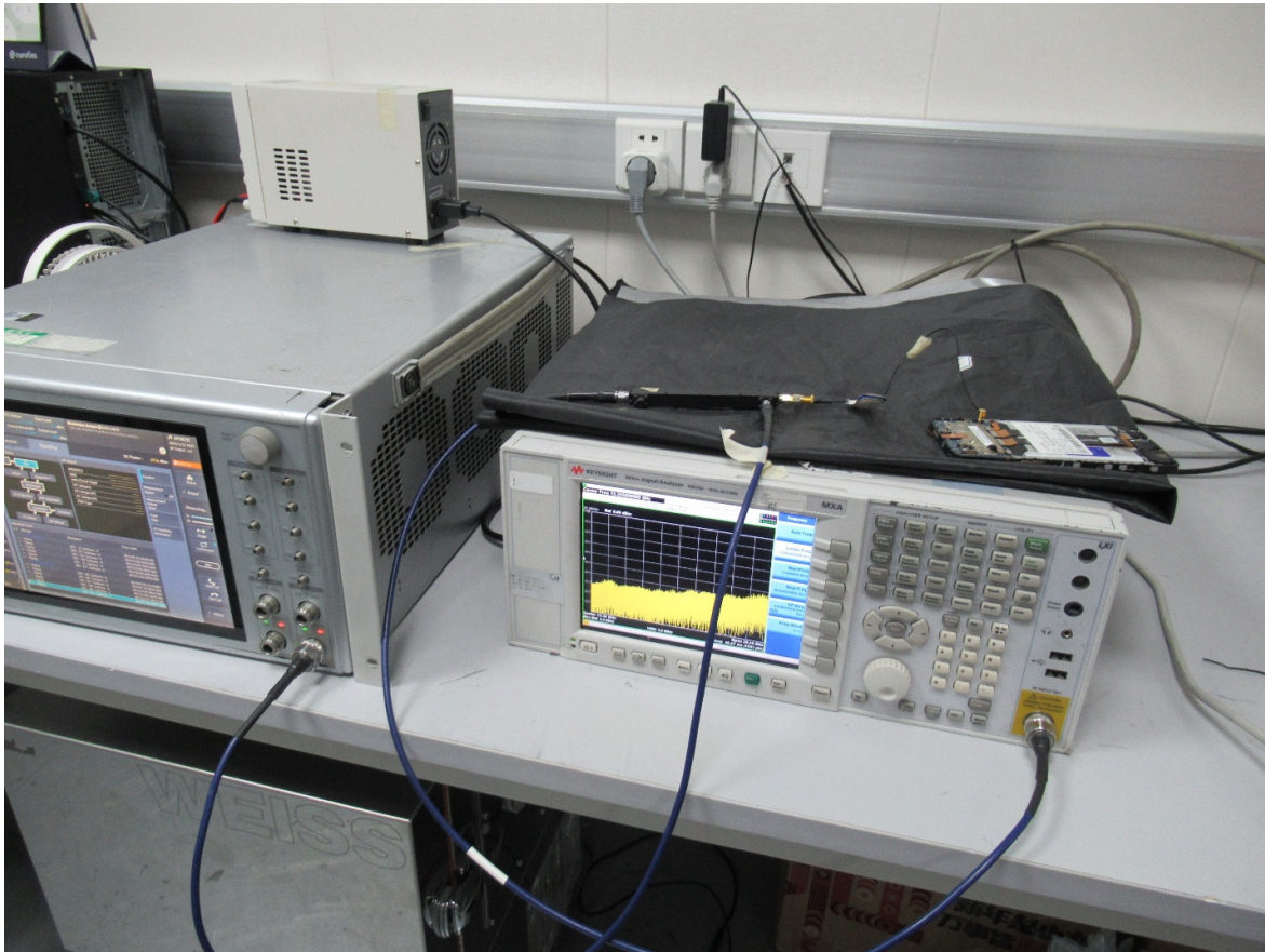
WWAN Test Setup
