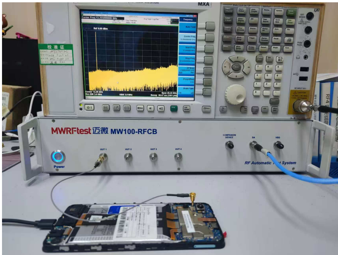
WLAN Test Setup
