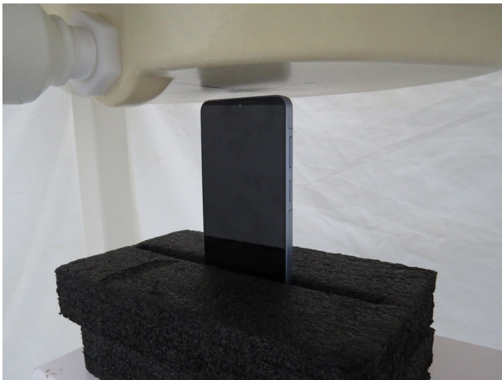
Picture 9: Top Edge, the distance from EUT to the bottom of the Phantom is 5mm
