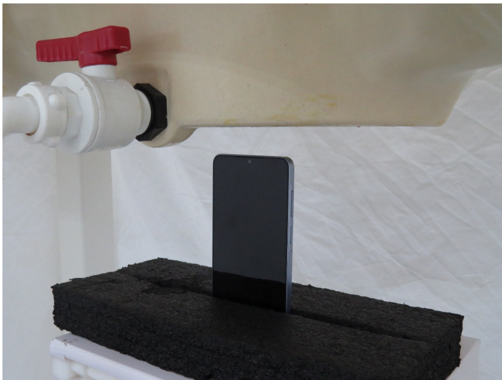
Picture 21: Top Edge, the distance from EUT to the bottom of the Phantom is 24mm
