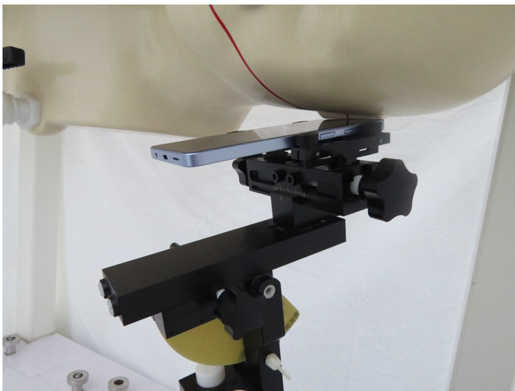
Picture 2: Left Tilt 15 Degree Position
