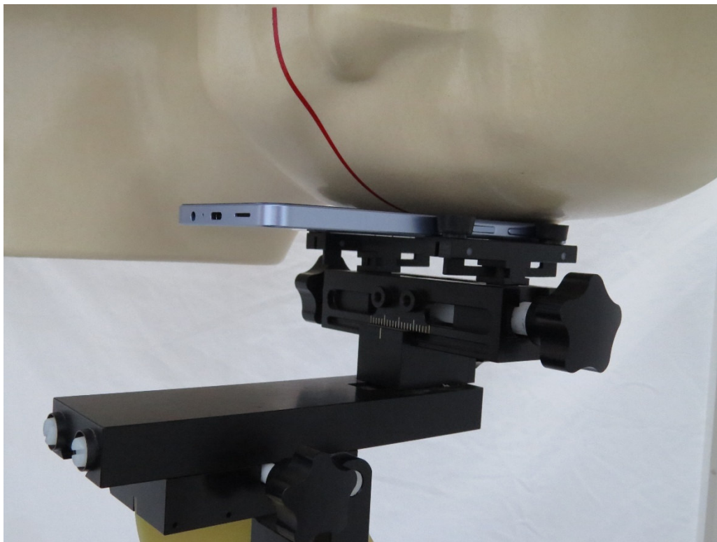
Picture 1: Left Cheek Position
