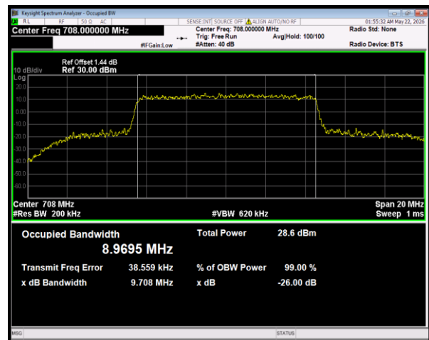
Band28(703-716) 64QAM BW=10MHz Channel=27260 RB Size=50 Position=#0
