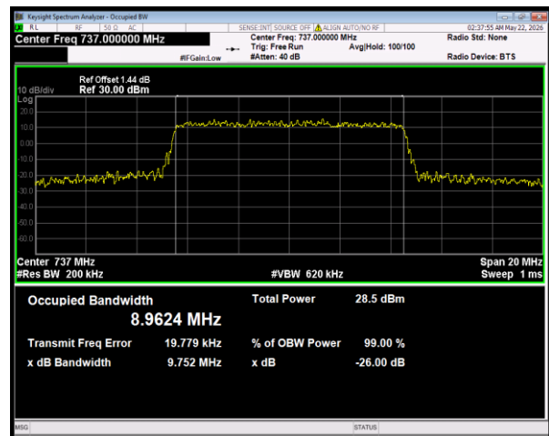
Band28(728-746) 64QAM BW=10MHz Channel=27550 RB Size=50 Position=#0
