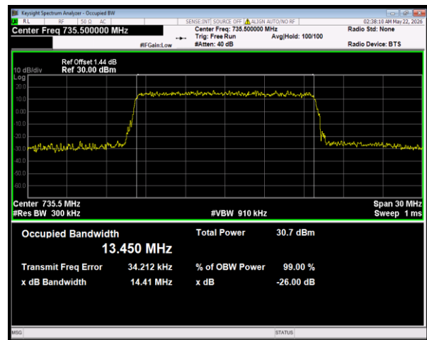
Band28(728-746) QPSK BW=15MHz Channel=27535 RB Size=75 Position=#0
