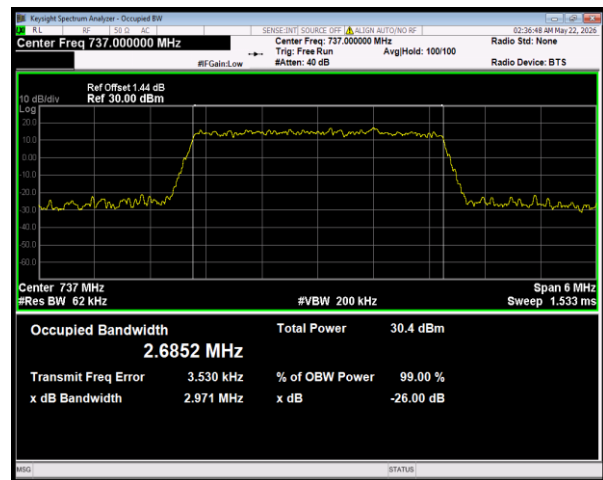
Band28(728-746) QPSK BW=3MHz Channel=27550 RB Size=15 Position=#0
