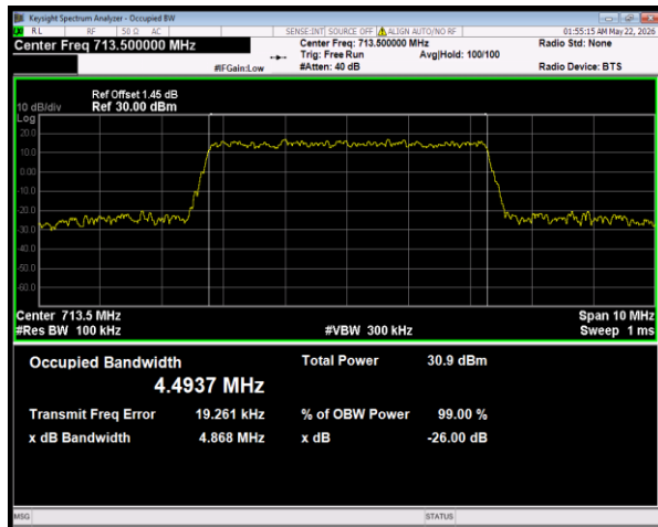
Band28(703-716) QPSK BW=5MHz Channel=27315 RB Size=25 Position=#0
