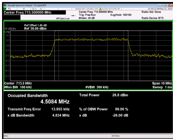
Band28(703-716) 64QAM BW=5MHz Channel=27315 RB Size=25 Position=#0
