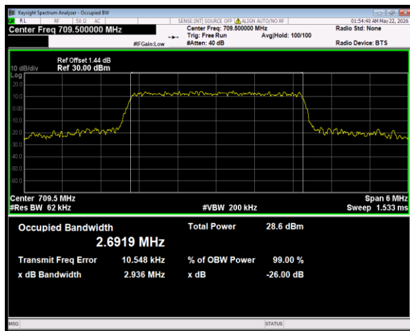
Band28(703-716) 64QAM BW=3MHz Channel=27275 RB Size=15 Position=#0
