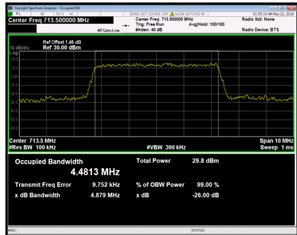
Band28(703-716) 16QAM BW=5MHz Channel=27315 RB Size=25 Position=#0
