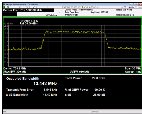
Band28(728-746) 16QAM BW=15MHz Channel=27535 RB Size=75 Position=#0
