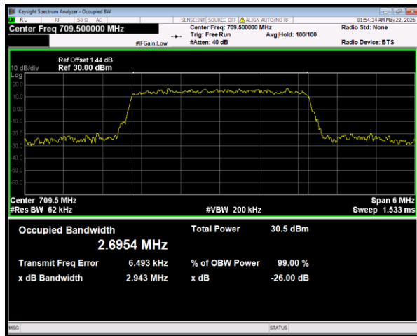
Band28(703-716) QPSK BW=3MHz Channel=27275 RB Size=15 Position=#0
