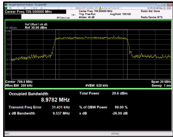
Band28(703-716) 16QAM BW=10MHz Channel=27275 RB Size=50 Position=#0
