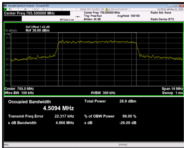
Band28(703-716) 64QAM BW=5MHz Channel=27235 RB Size=25 Position=#0
