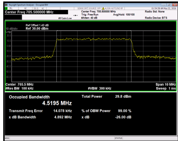
Band28(703-716) 16QAM BW=5MHz Channel=27235 RB Size=25 Position=#0
