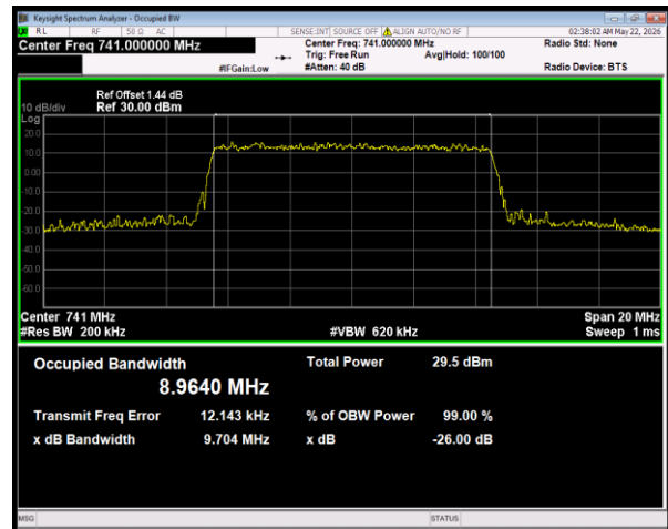
Band28(728-746) 16QAM BW=10MHz Channel=27590 RB Size=50 Position=#0
