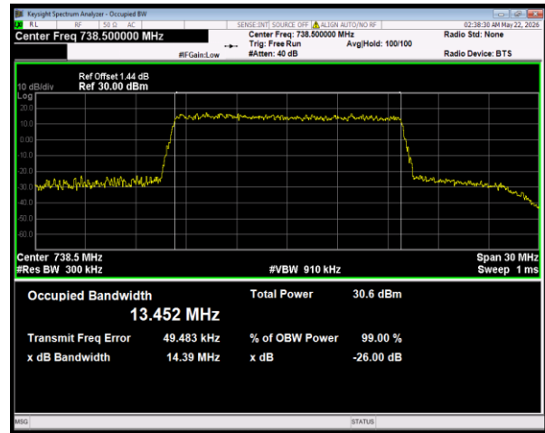
Band28(728-746) QPSK BW=15MHz Channel=27565 RB Size=75 Position=#0
