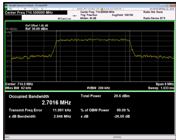
Band28(703-716) 64QAM BW=3MHz Channel=27325 RB Size=15 Position=#0
