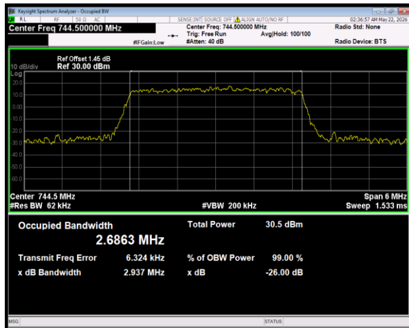
Band28(728-746) QPSK BW=3MHz Channel=27625 RB Size=15 Position=#0
