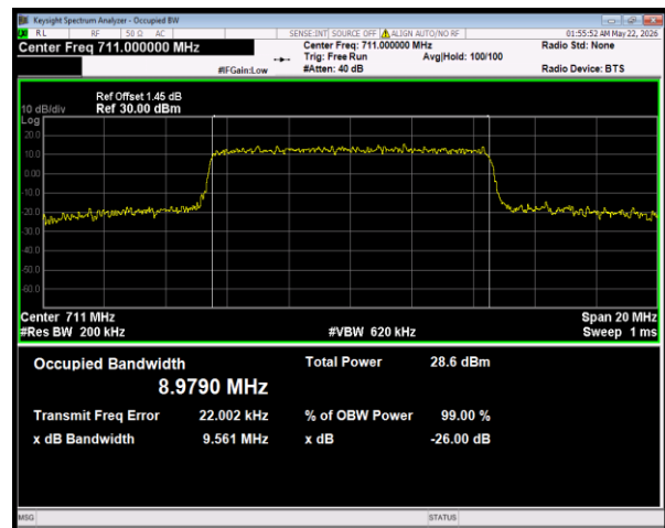
Band28(703-716) 64QAM BW=10MHz Channel=27290 RB Size=50 Position=#0
