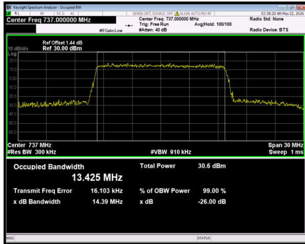
Band28(728-746) QPSK BW=15MHz Channel=27550 RB Size=75 Position=#0
