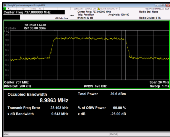
Band28(728-746) 16QAM BW=10MHz Channel=27550 RB Size=50 Position=#0
