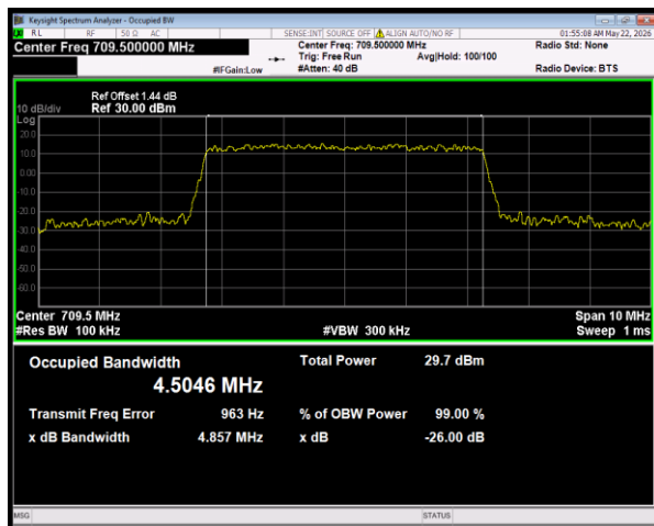
Band28(703-716) 16QAM BW=5MHz Channel=27275 RB Size=25 Position=#0
