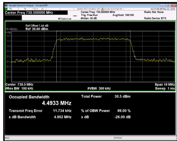
Band28(728-746) QPSK BW=5MHz Channel=27485 RB Size=25 Position=#0
