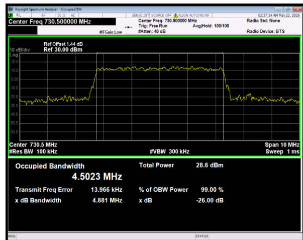
Band28(728-746) 64QAM BW=5MHz Channel=27485 RB Size=25 Position=#0
