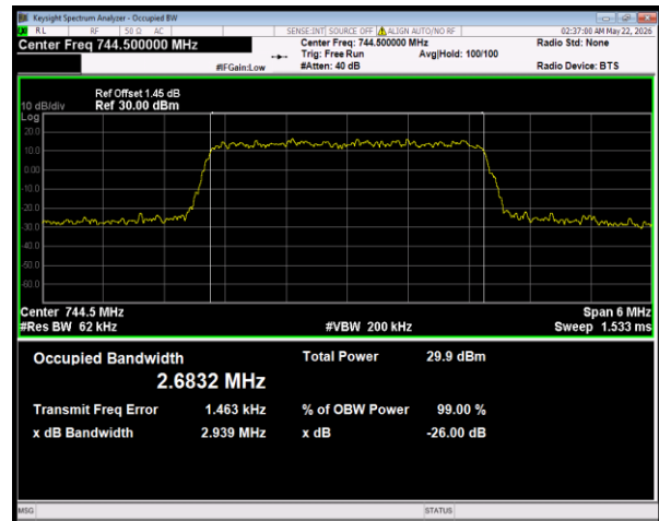
Band28(728-746) 16QAM BW=3MHz Channel=27625 RB Size=15 Position=#0
