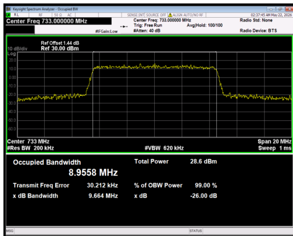
Band28(728-746) 64QAM BW=10MHz Channel=27510 RB Size=50 Position=#0
