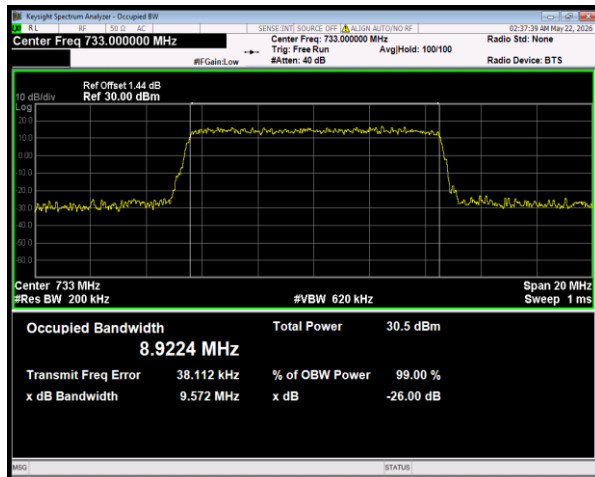
Band28(728-746) QPSK BW=10MHz Channel=27510 RB Size=50 Position=#0
