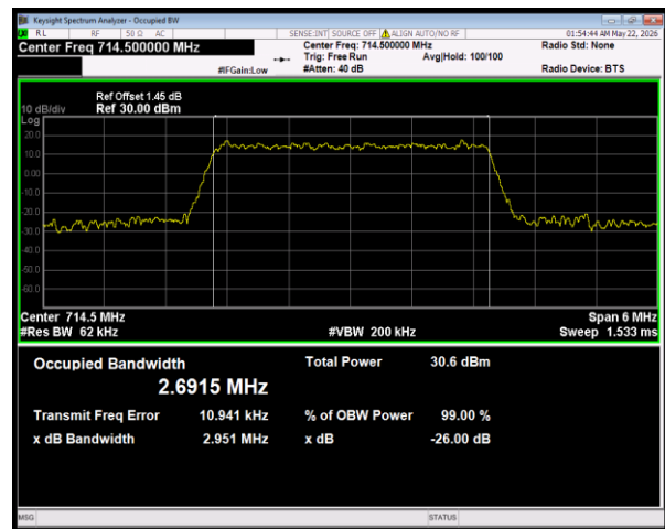
Band28(703-716) QPSK BW=3MHz Channel=27325 RB Size=15 Position=#0
