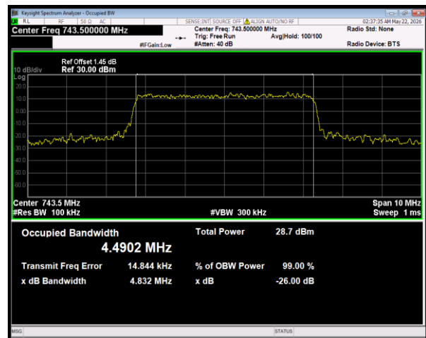
Band28(728-746) 64QAM BW=5MHz Channel=27615 RB Size=25 Position=#0
