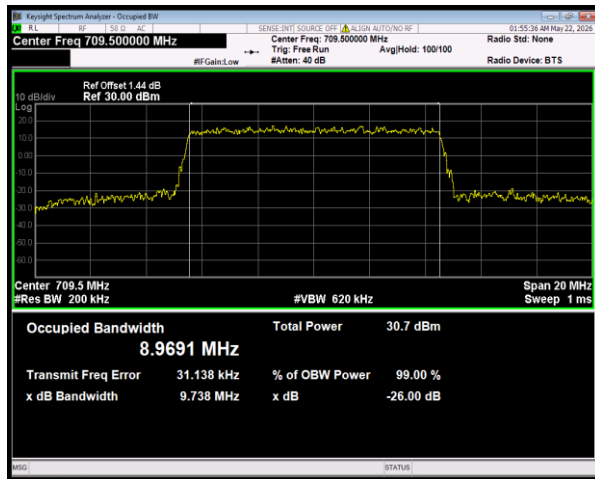
Band28(703-716) QPSK BW=10MHz Channel=27275 RB Size=50 Position=#0
