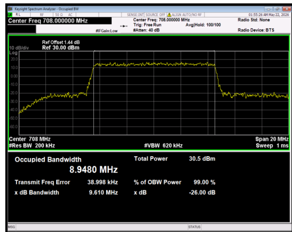
Band28(703-716) QPSK BW=10MHz Channel=27260 RB Size=50 Position=#0
