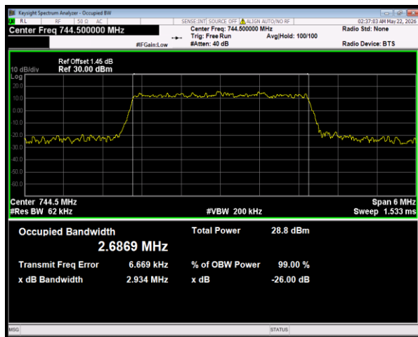
Band28(728-746) 64QAM BW=3MHz Channel=27625 RB Size=15 Position=#0
