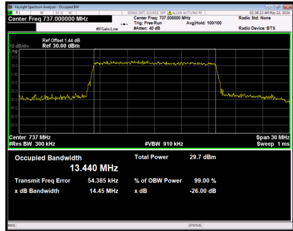
Band28(728-746) 16QAM BW=15MHz Channel=27550 RB Size=75 Position=#0
