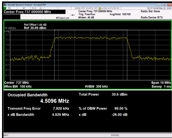
Band28(728-746) QPSK BW=5MHz Channel=27550 RB Size=25 Position=#0
