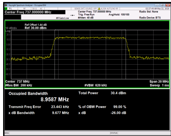
Band28(728-746) QPSK BW=10MHz Channel=27550 RB Size=50 Position=#0
