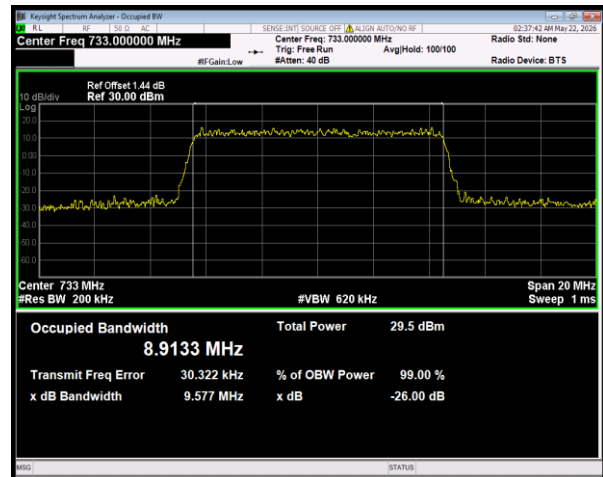
Band28(728-746) 16QAM BW=10MHz Channel=27510 RB Size=50 Position=#0
