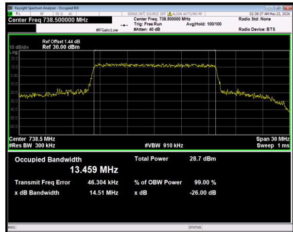
Band28(728-746) 64QAM BW=15MHz Channel=27565 RB Size=75 Position=#0
