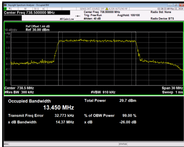
Band28(728-746) 16QAM BW=15MHz Channel=27565 RB Size=75 Position=#0
