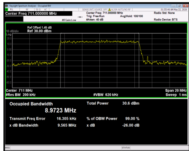
Band28(703-716) QPSK BW=10MHz Channel=27290 RB Size=50 Position=#0
