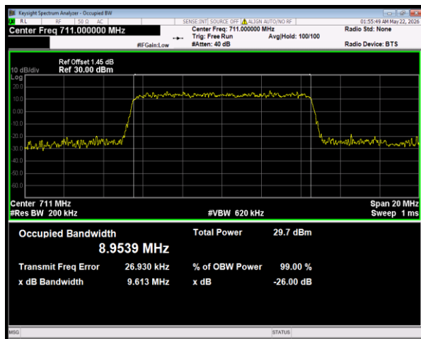
Band28(703-716) 16QAM BW=10MHz Channel=27290 RB Size=50 Position=#0
