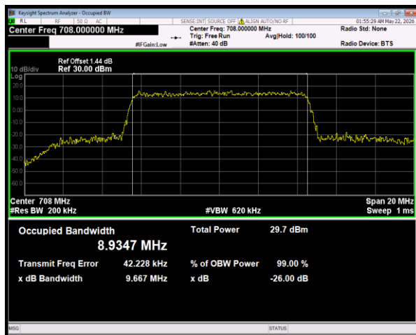
Band28(703-716) 16QAM BW=10MHz Channel=27260 RB Size=50 Position=#0
