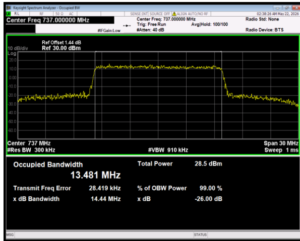
Band28(728-746) 64QAM BW=15MHz Channel=27550 RB Size=75 Position=#0
