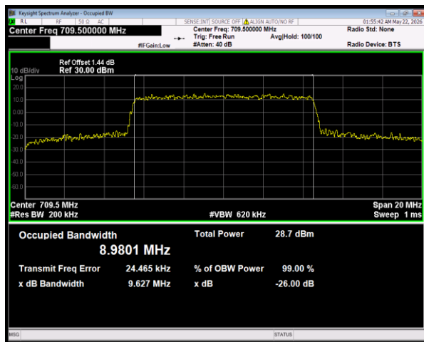
Band28(703-716) 64QAM BW=10MHz Channel=27275 RB Size=50 Position=#0
