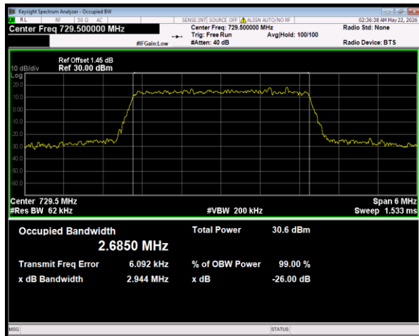
Band28(728-746) QPSK BW=3MHz Channel=27475 RB Size=15 Position=#0
