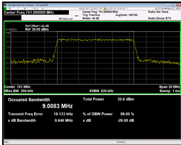
Band28(728-746) QPSK BW=10MHz Channel=27590 RB Size=50 Position=#0
