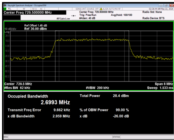
Band28(728-746) 64QAM BW=3MHz Channel=27475 RB Size=15 Position=#0
