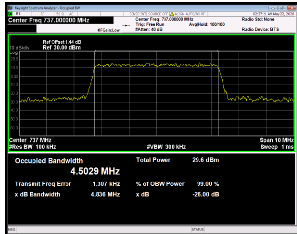
Band28(728-746) 16QAM BW=5MHz Channel=27550 RB Size=25 Position=#0
