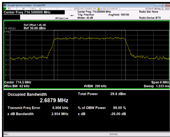
Band28(703-716) 16QAM BW=3MHz Channel=27325 RB Size=15 Position=#0
