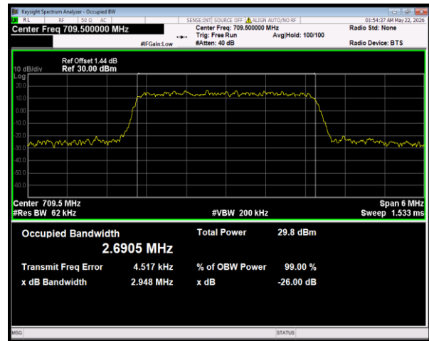
Band28(703-716) 16QAM BW=3MHz Channel=27275 RB Size=15 Position=#0
