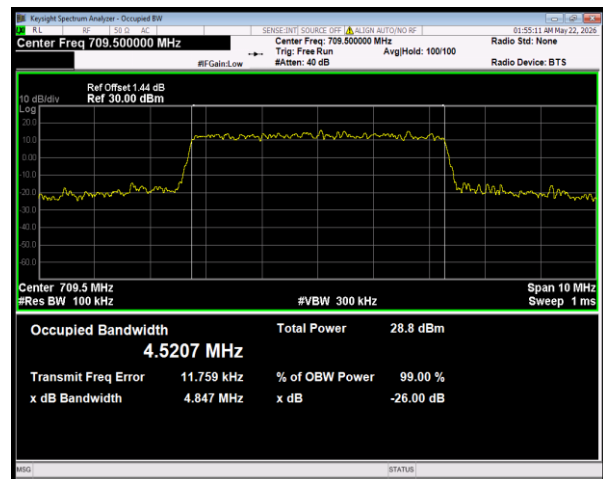
Band28(703-716) 64QAM BW=5MHz Channel=27275 RB Size=25 Position=#0
