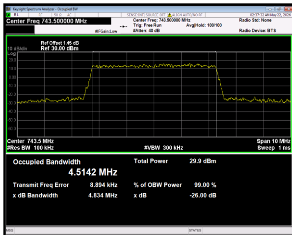
Band28(728-746) 16QAM BW=5MHz Channel=27615 RB Size=25 Position=#0
