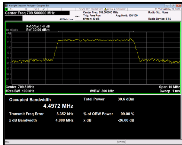
Band28(703-716) QPSK BW=5MHz Channel=27275 RB Size=25 Position=#0
