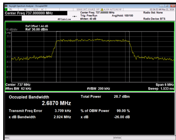
Band28(728-746) 64QAM BW=3MHz Channel=27550 RB Size=15 Position=#0
