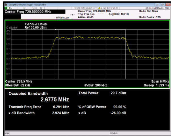
Band28(728-746) 16QAM BW=3MHz Channel=27475 RB Size=15 Position=#0
