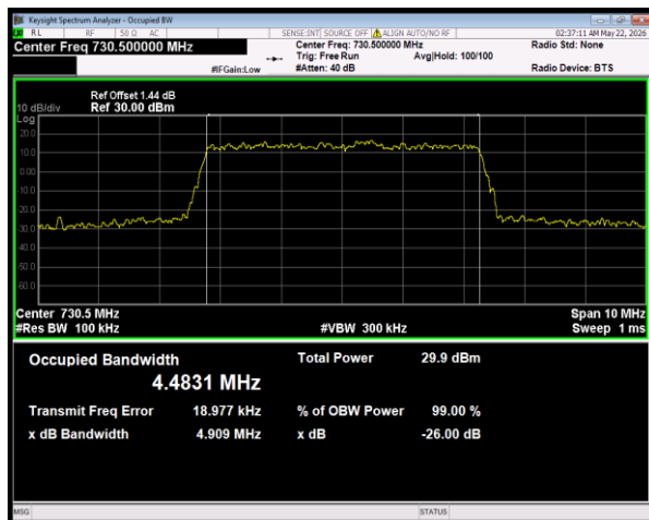
Band28(728-746) 16QAM BW=5MHz Channel=27485 RB Size=25 Position=#0
