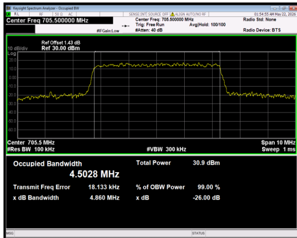
Band28(703-716) QPSK BW=5MHz Channel=27235 RB Size=25 Position=#0
