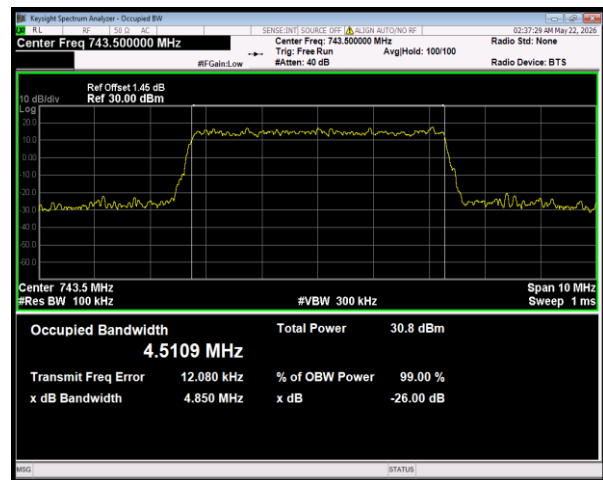
Band28(728-746) QPSK BW=5MHz Channel=27615 RB Size=25 Position=#0
