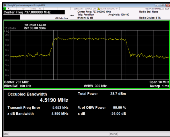
Band28(728-746) 64QAM BW=5MHz Channel=27550 RB Size=25 Position=#0
