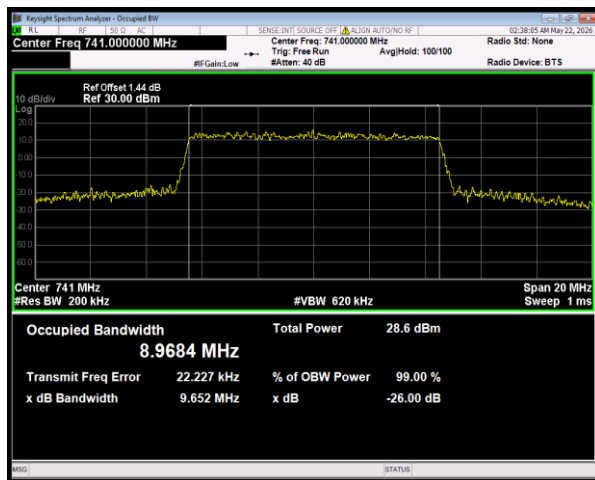
Band28(728-746) 64QAM BW=10MHz Channel=27590 RB Size=50 Position=#0
