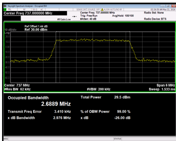
Band28(728-746) 16QAM BW=3MHz Channel=27550 RB Size=15 Position=#0
