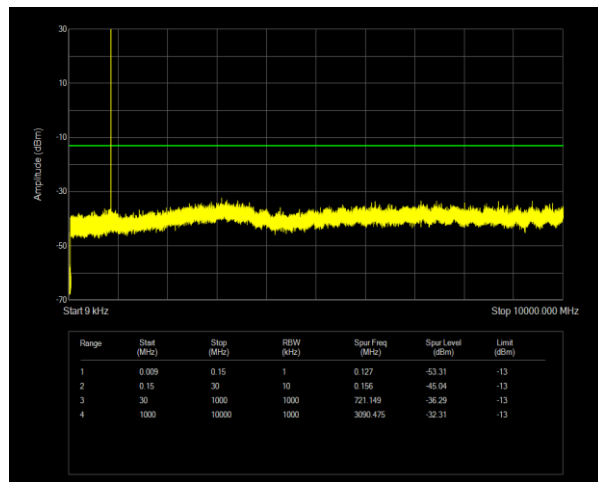
GPRS850 Channel=251 NVNT
