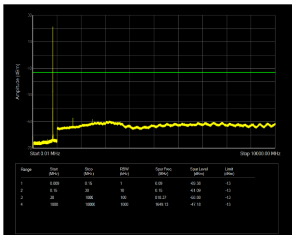
Band26(824-849) QPSK BW=1.4MHz Channel=26797 RB Size=1 Position=#0
