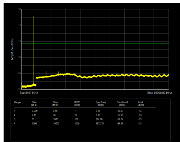
Band26(824-849) QPSK BW=1.4MHz Channel=26915 RB Size=1 Position=#0
