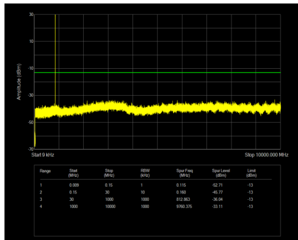
EGPRS850 Channel=251 NVNT
