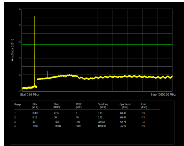
Band26(824-849) QPSK BW=3MHz Channel=27025 RB Size=1 Position=#0
