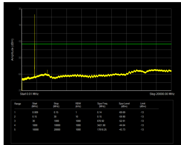
Band4 QPSK BW=10MHz Channel=20000 RB Size=1 Position=#0
