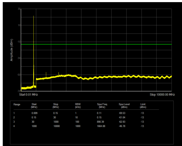
Band26(824-849) QPSK BW=10MHz Channel=26915 RB Size=1 Position=#0
