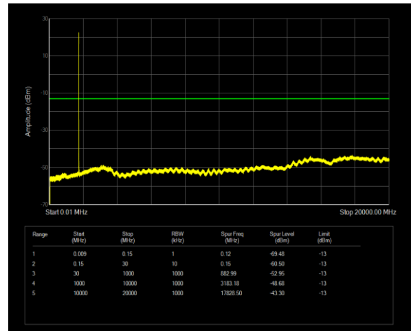
Band4 QPSK BW=1.4MHz Channel=20175 RB Size=1 Position=#0
