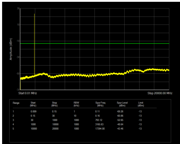
Band2 QPSK BW=1.4MHz Channel=19193 RB Size=1 Position=#0
