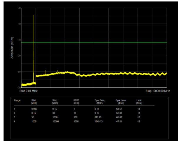
Band26(824-849) QPSK BW=3MHz Channel=26805 RB Size=1 Position=#0
