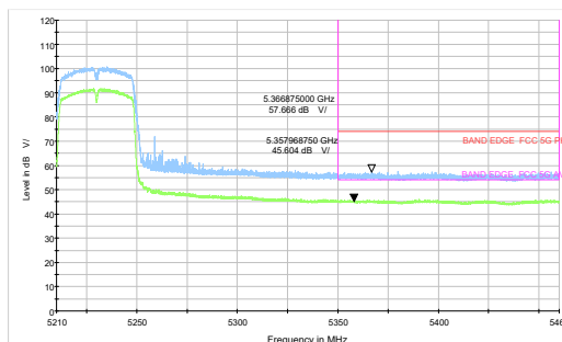
802.11ac VHT40-Channel 46: Peak + Average
