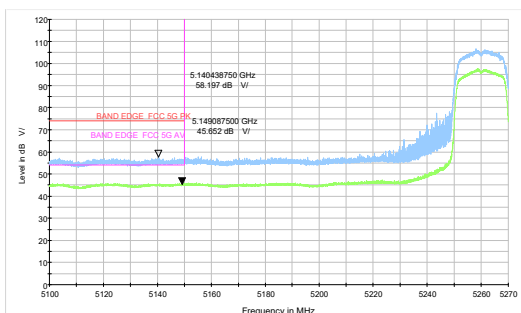
802.11ac VHT20 -Channel 52: Peak + Average
