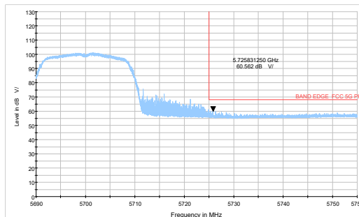
802.11ac VHT20-Channel 140: Peak
