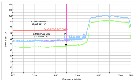
802.11ac VHT40-Channel 38: Peak + Average
