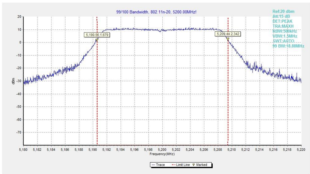
Fig.93 99% Occupied bandwidth (802.11n-HT20, 5200MHz)
