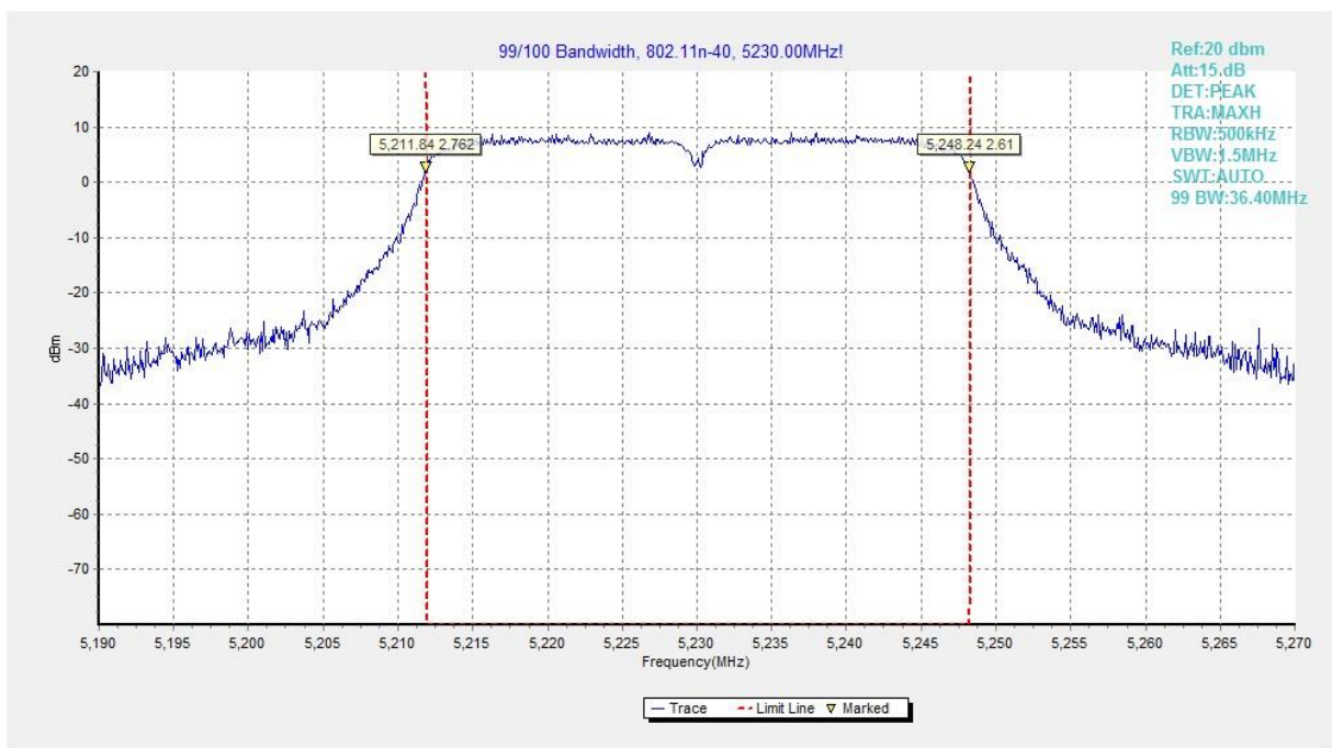
Fig.99 99% Occupied bandwidth (802.11n-HT40, 5230MHz)
