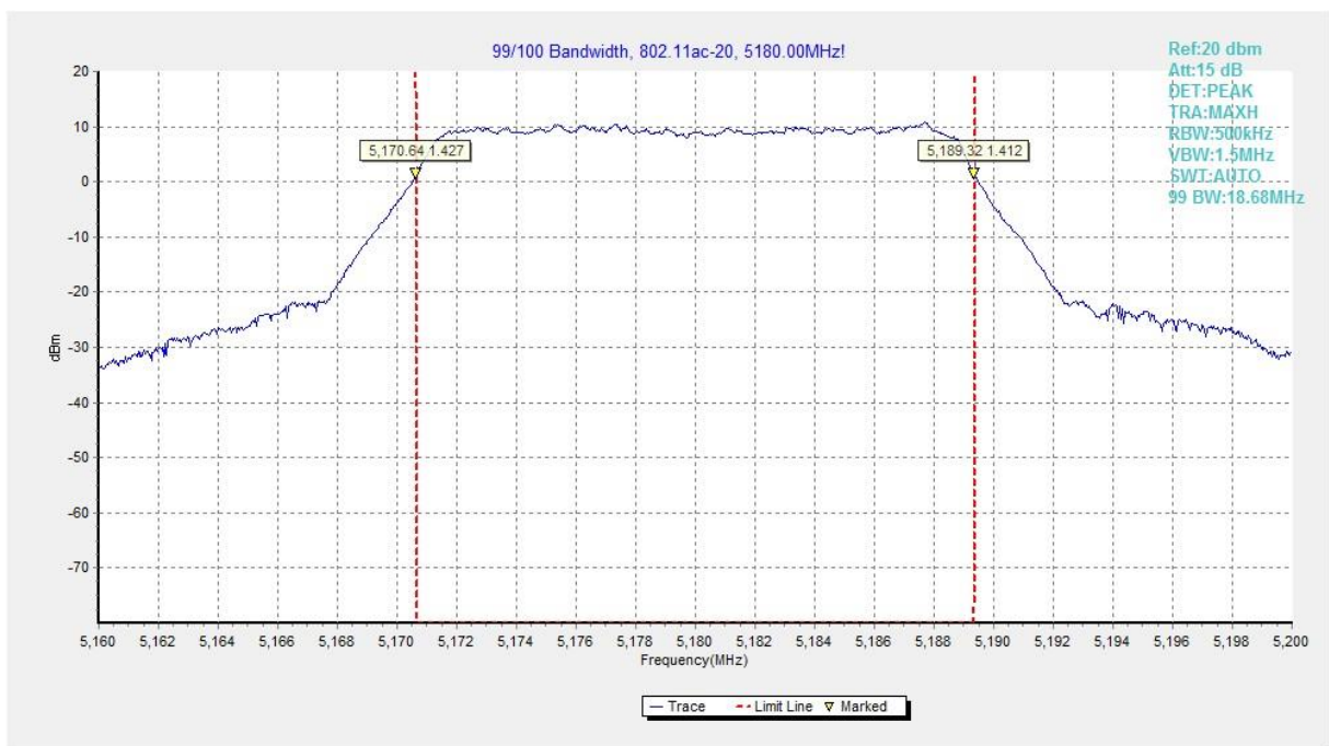
Fig.95 99% Occupied bandwidth (802.11ac-HT20, 5180MHz)
