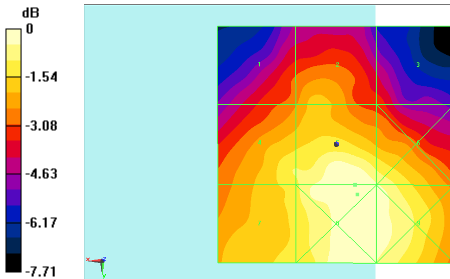
Fig B.6 HAC RF E-Field WIFI2.4G
