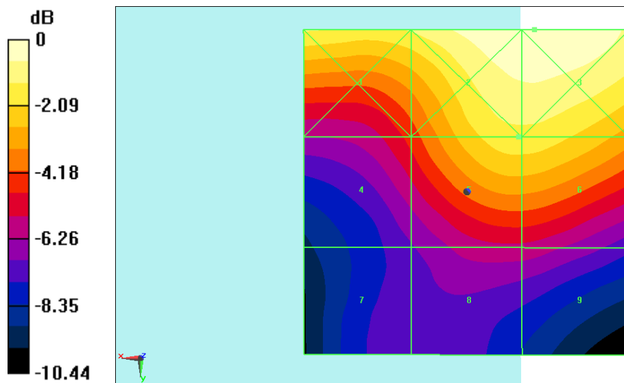
Fig B.4 HAC RF E-Field LTE Band41 PC3 QPSK
