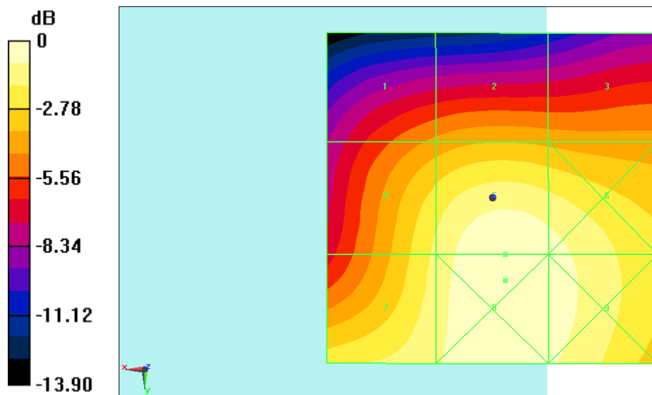
Fig B.5 HAC RF E-Field LTE Band48 QPSK
