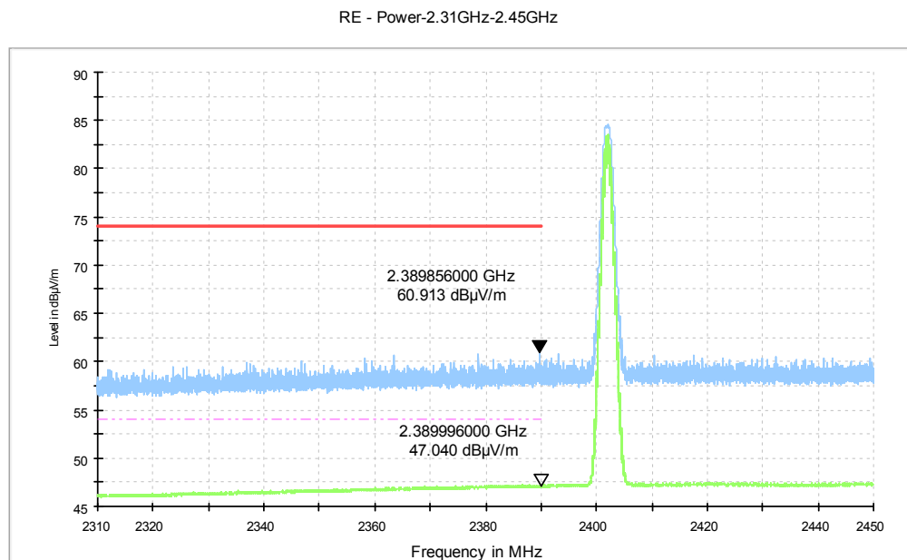
Fig.3. Frequency Band Edges: GFSK, Channel 0, 2.31 GHz – 2.45GHz
