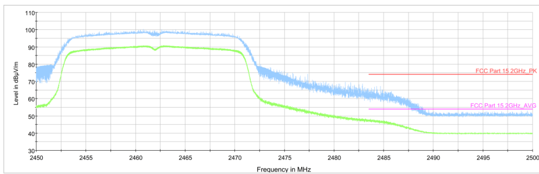
Fig.A.6.2.6 Transmitter Spurious Emission - Radiated (Power): 802.11n-HT20, ch11, 2.45 GHz - 2.50GHz
