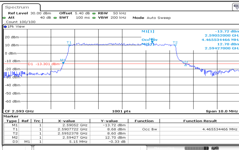
Band41-5MHz-QPSK-40620-25RB#0-4.466
