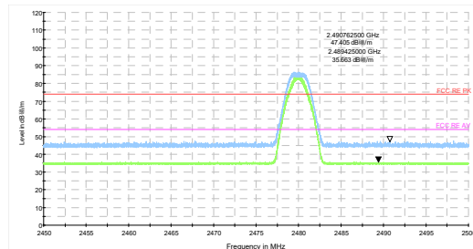
Bluetooth LE Channel 39 Peak+ Average-2M
