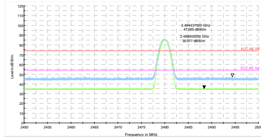
Bluetooth LE Channel 39 Peak+ Average-1M
