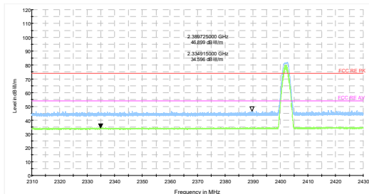
Bluetooth LE Channel 0 Peak+ Average-2M
