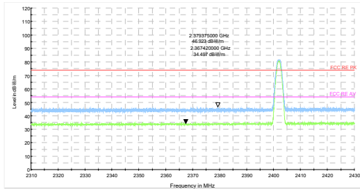
Bluetooth LE Channel 0 Peak+ Average-1M
