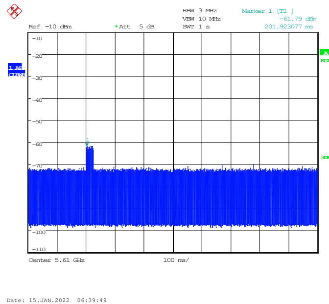
Fig.A.1 80M Calibration Result
