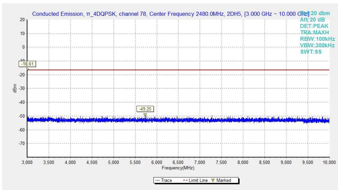
Fig.41. Conducted \pi/4 DQPSK, Channel 78, 3GHz - 10GHz
