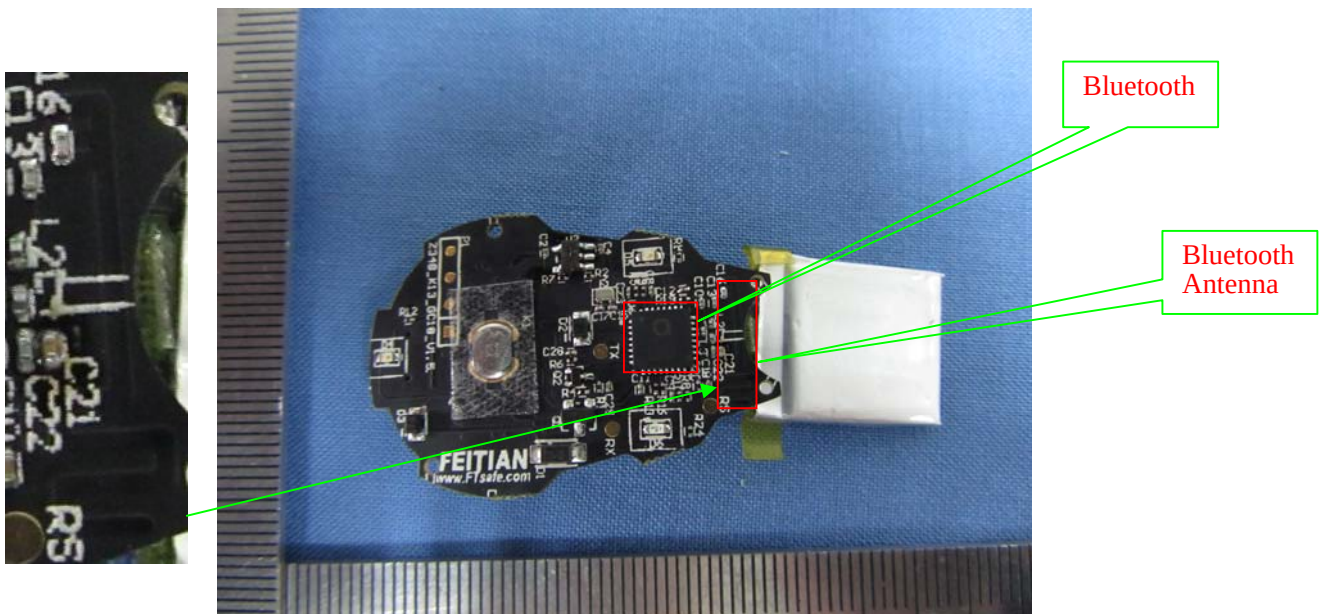
EUT – Mainboard Top View
