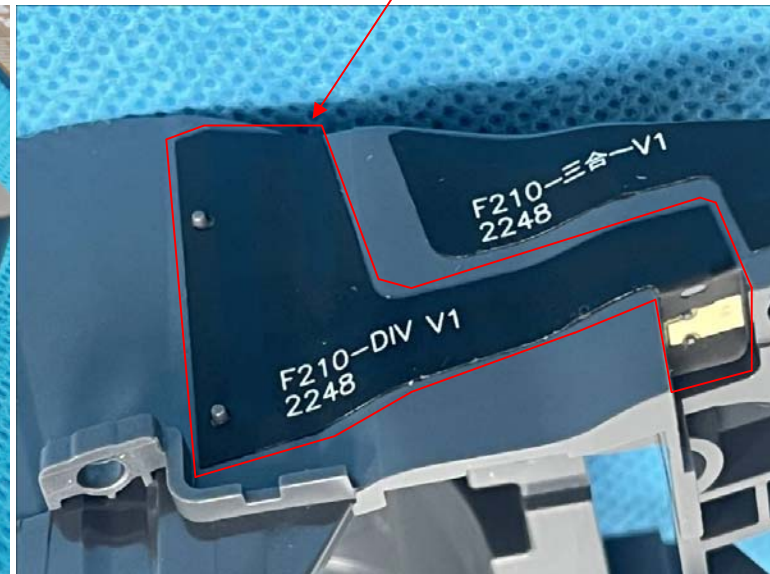
DIV Antenna
