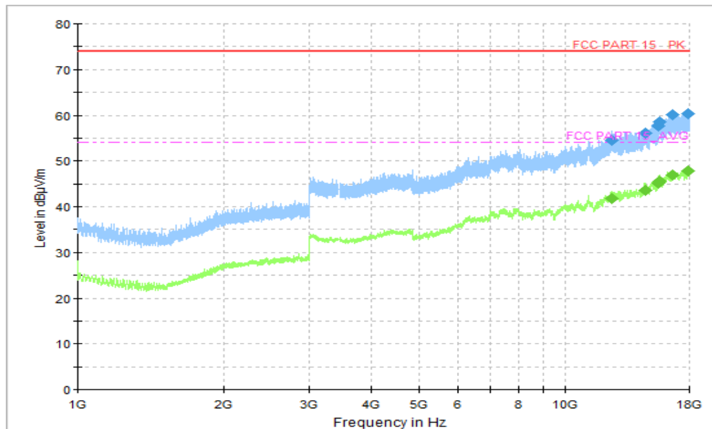
Figure A.1.8. Radiated Emission (WCDMA receiver Band 5, 1GHz to 18GHz) Final_Results_PK
