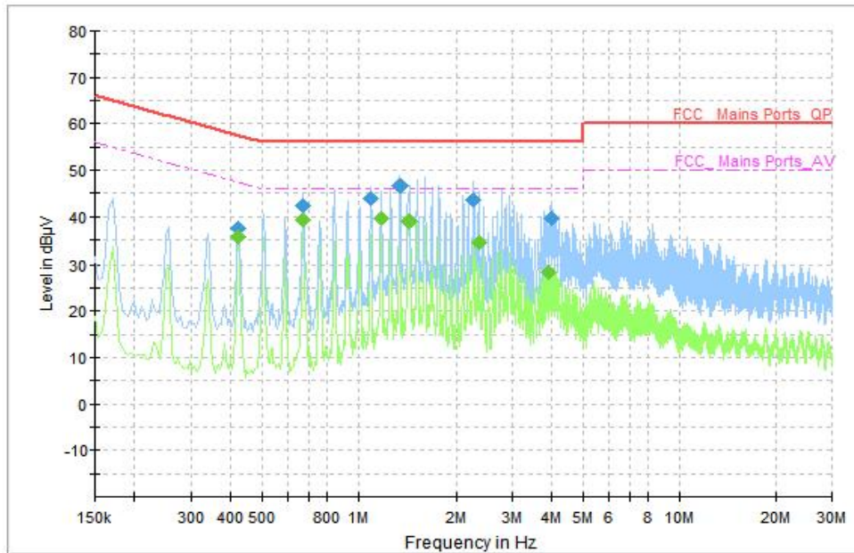
Fig.26 AC Power line Conducted Emission (Idle, AE3, 120V), 1M
