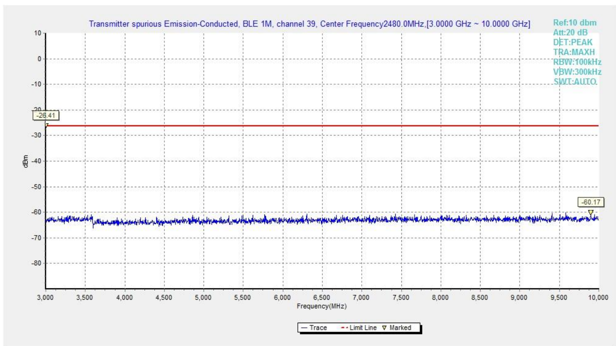
Fig.14 Conducted Spurious Emission (Ch39, 3GHz-10GHz), LE 1M
