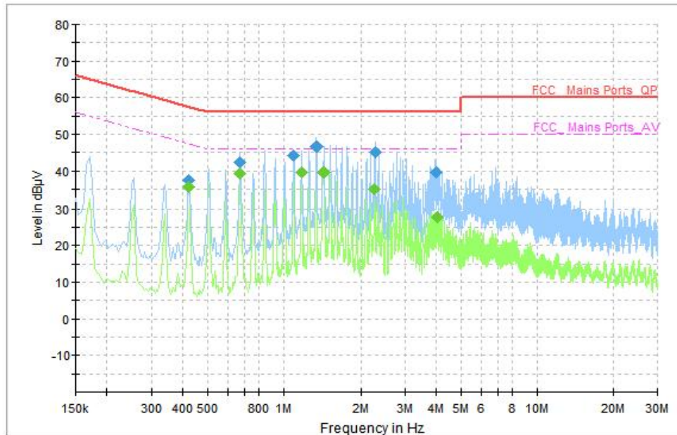
Fig.25 AC Power line Conducted Emission (Traffic, AE3, 120V), 1M
