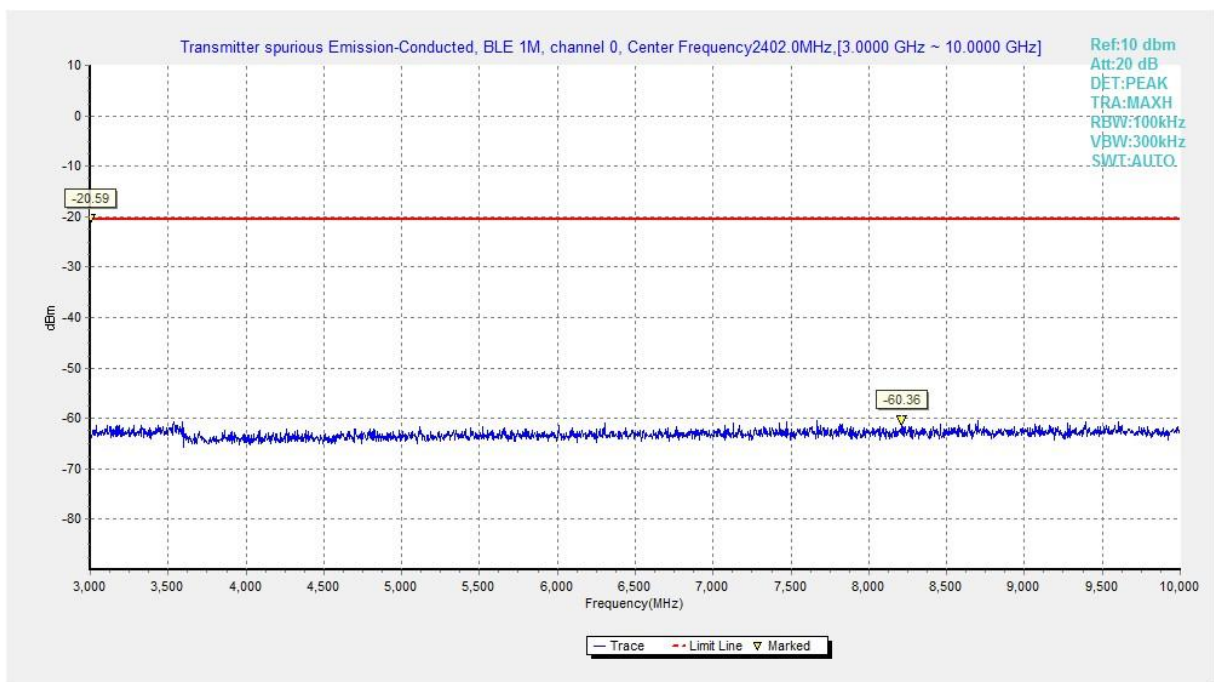
Fig.10 Conducted Spurious Emission (Ch0, 3GHz-10GHz), LE 1M
