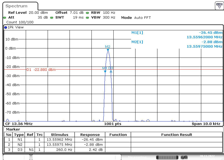
Figure A-4 20dB Bandwidth
